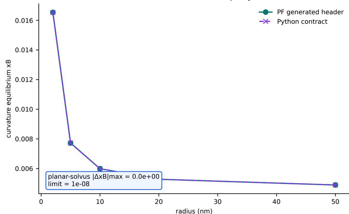
Gibbs-Thomson / solvus parity
