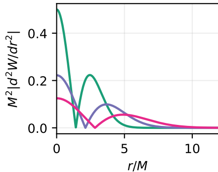
second derivative
