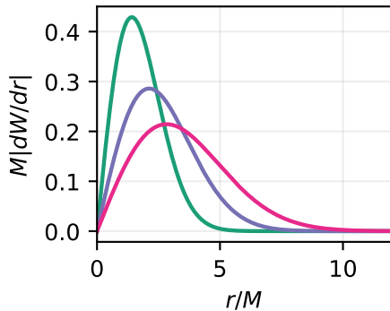
first derivative
