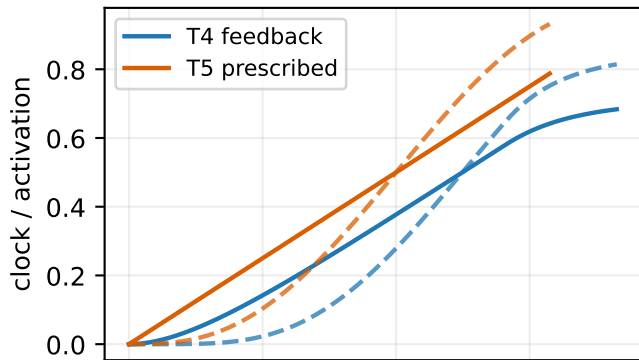
Relative boost diagnostic
