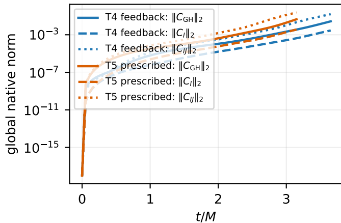
GH, reduction, and curl constraints
