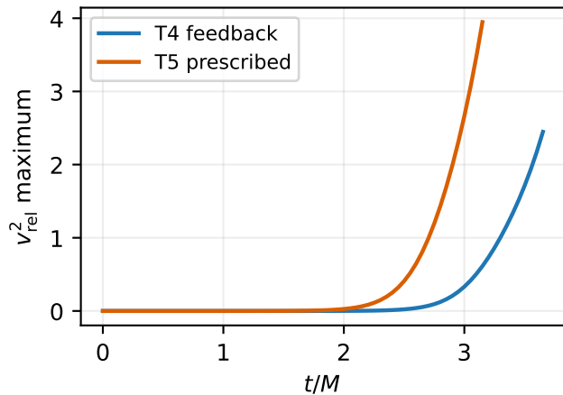
Relative boost diagnostic
