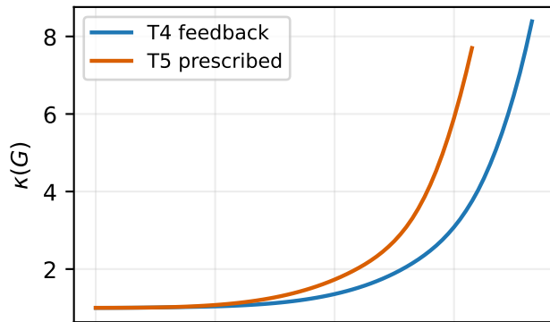
GH, reduction, and curl constraints
