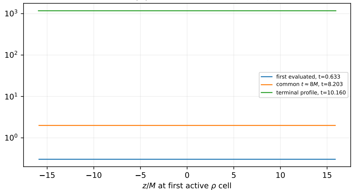
local |K| : axis-adjacent profile
