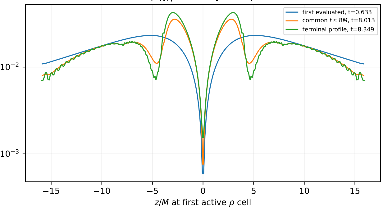
local |\nabla\chi|_\gamma : axis-adjacent profile
