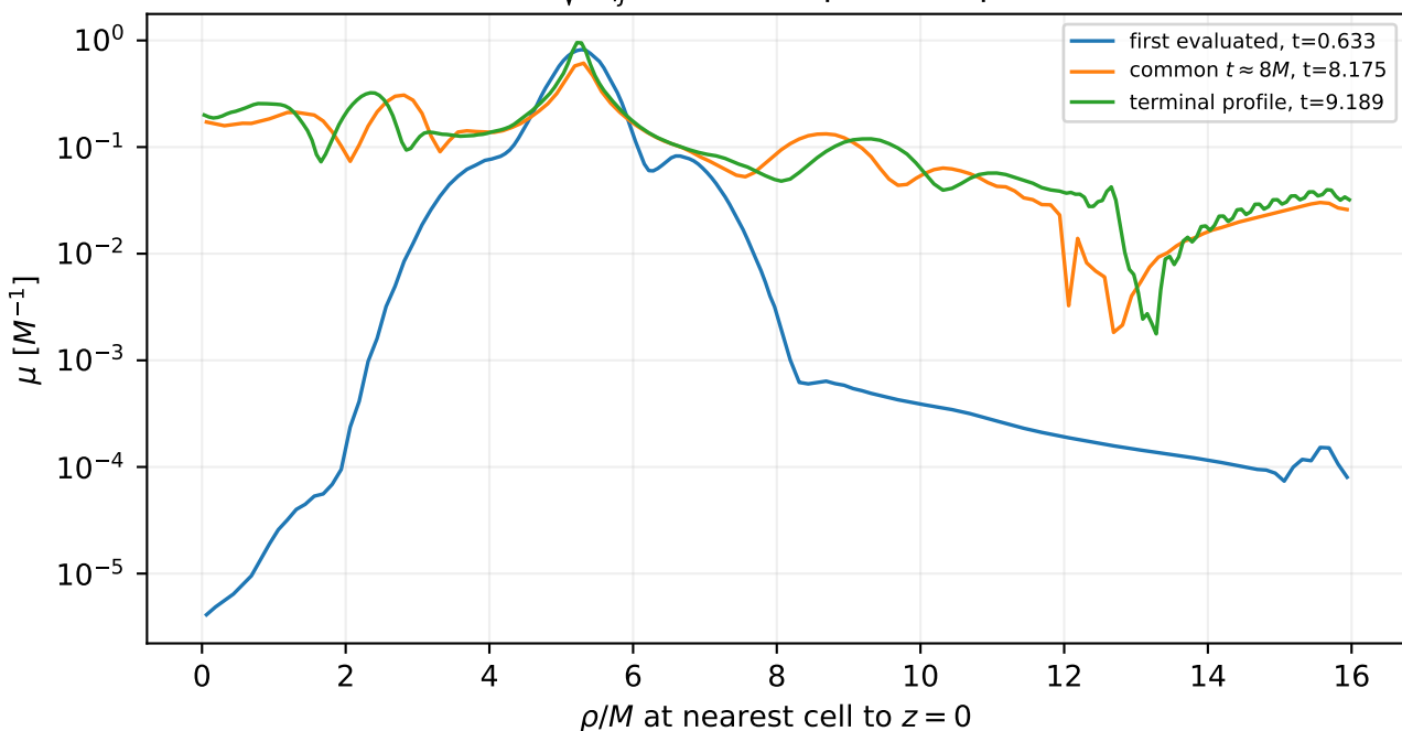
local |\nabla\chi|_\gamma : near-equatorial profile
