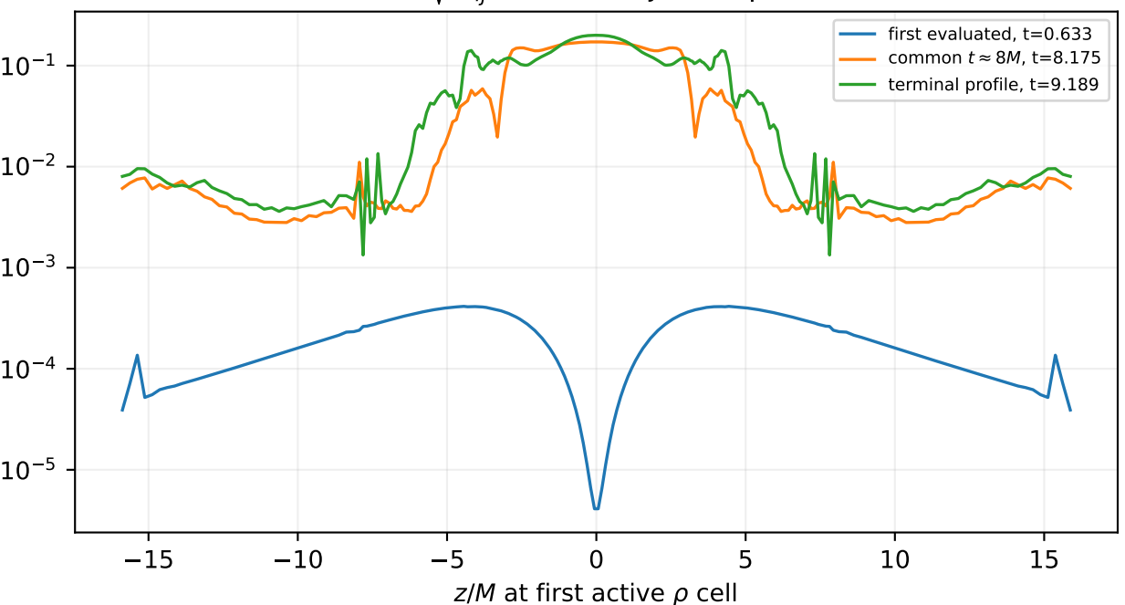
local |\nabla\chi|_\gamma : axis-adjacent profile
