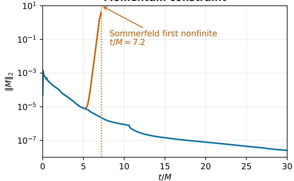
Momentum constraint
