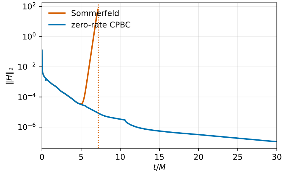
Hamiltonian constraint
