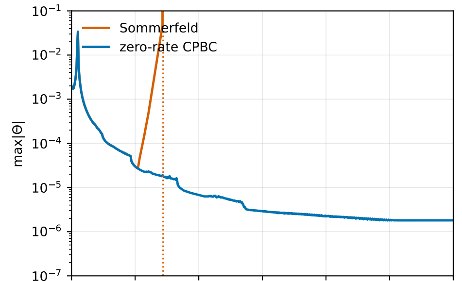
Thin-z no-sponge TDE gauge and constraint residual maxima
