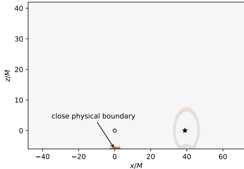
Sommerfeld at t/M = 7.00313
