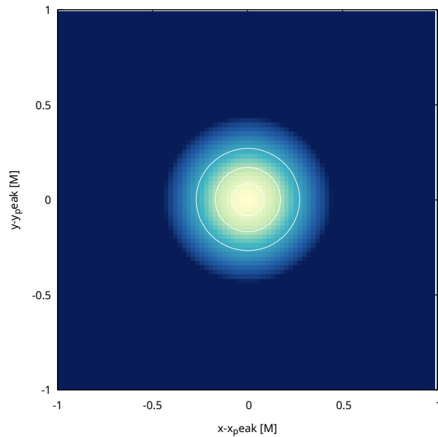
CPBC t=7.50234 M; \rho_{\text{max}}=1.233\text{e-}04 , R_1/2=0.085 , a/b=1.003
