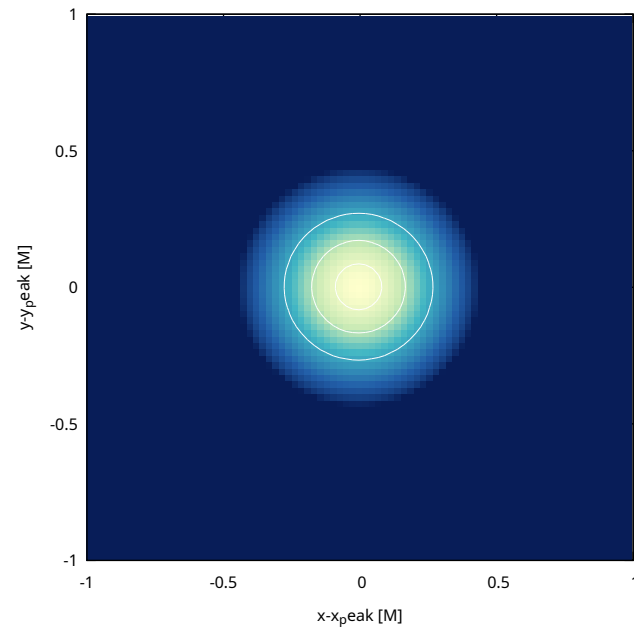
Sommerfeld t=7.00313 M; \rho_{\text{max}}=1.237\text{e-}04 , R_1/2=0.084 , a/b=1.017
