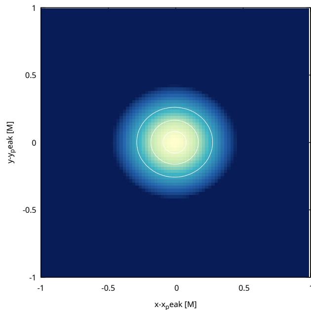
CPBC t=30.00000 M; \rho_{\text{max}}=1.287\text{e-}04 , R_1/2=0.083 , a/b=1.028
