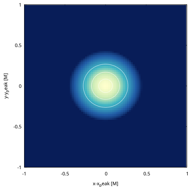
CPBC t=15.00120 M; \rho_{\text{max}}=1.249\text{e-}04 , R_1/2=0.084 , a/b=1.017
