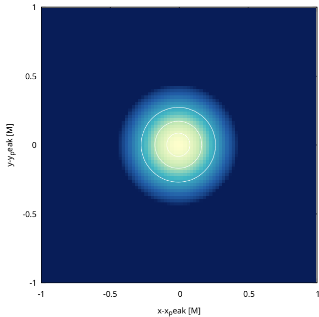
CPBC t=0.00000 M; \rho_{\text{max}}=1.227\text{e-}04 , R_1/2=0.084 , a/b=1.007
