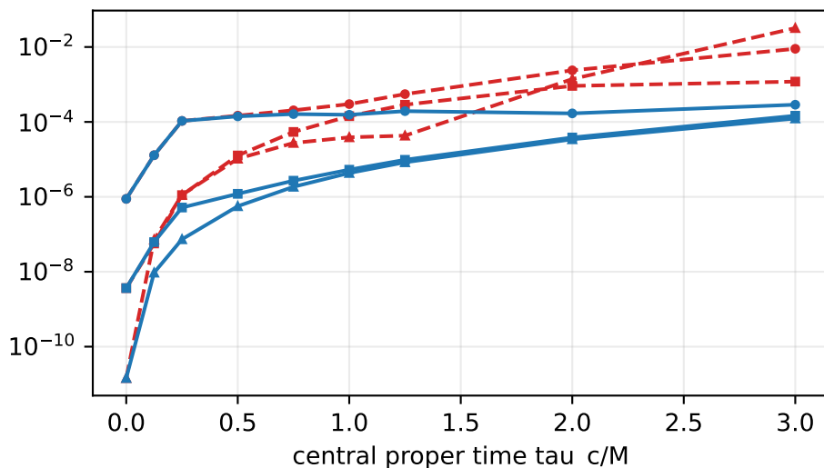
Z-norm2
