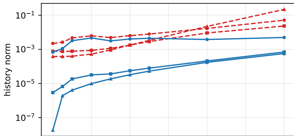
C-norm2
