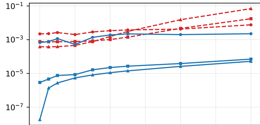
H-norm2
