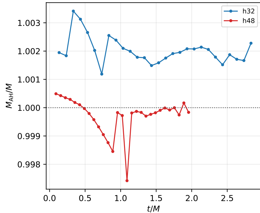
Accepted origin horizon mass
