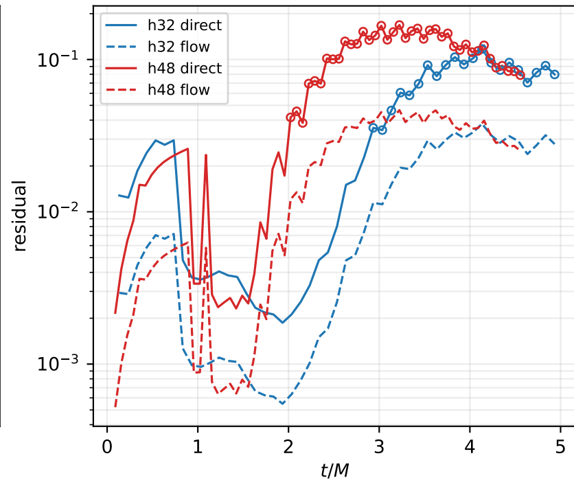
Origin finder residuals
