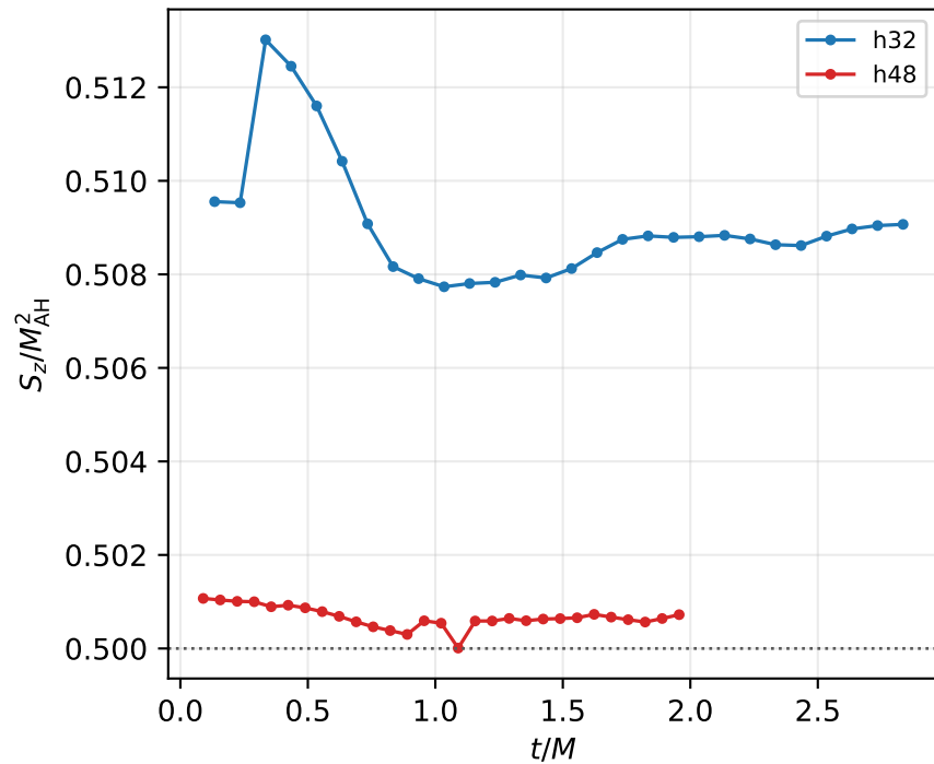
Accepted origin horizon spin
