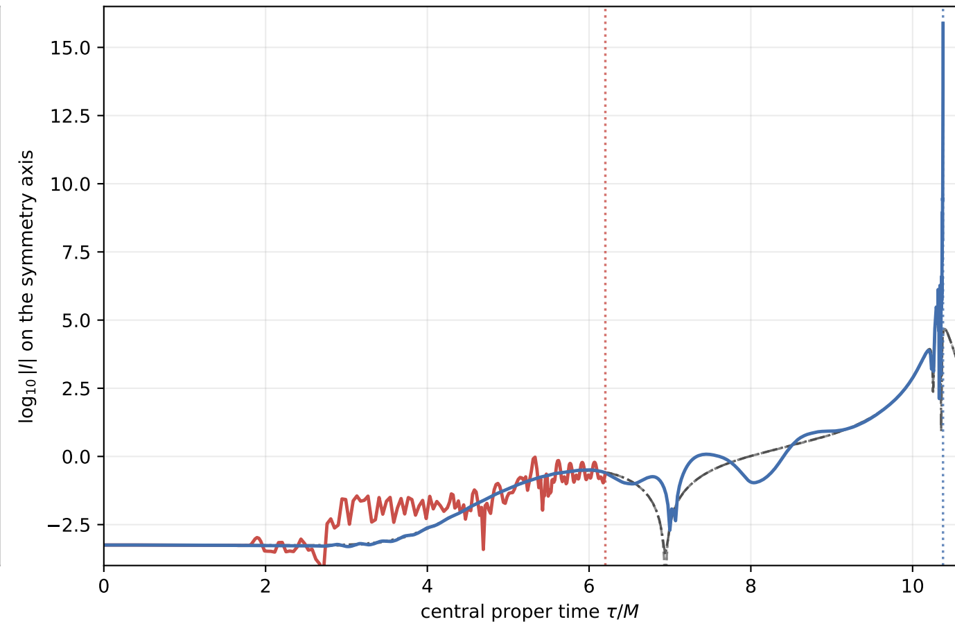
AthenaK diagnostic interval
