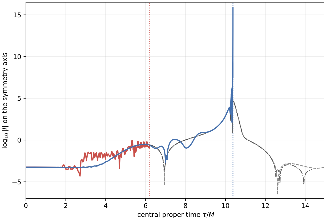
Published Figure-3 interval
