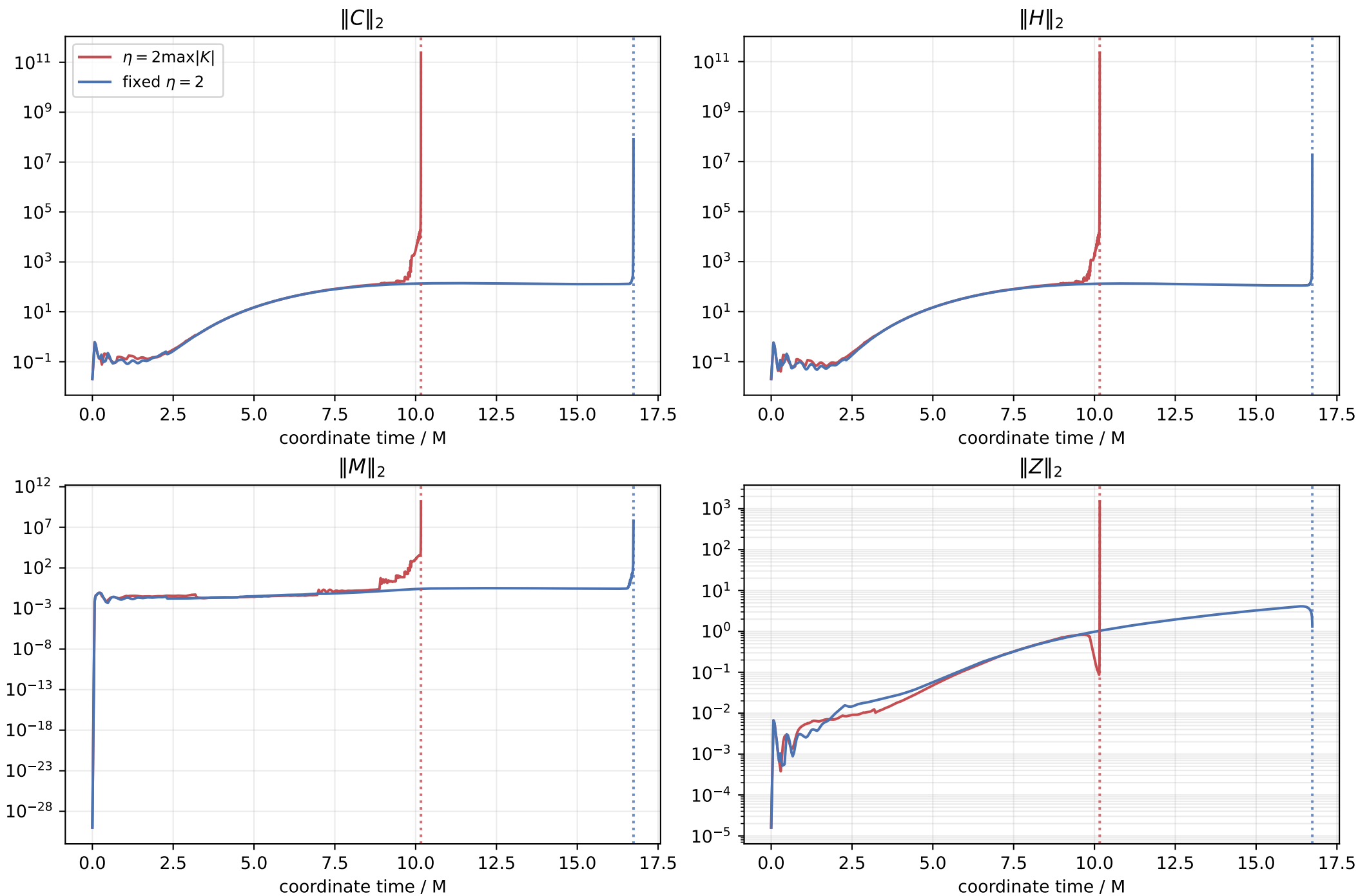
Figure-3 Brill diagnostic: constraint norms
