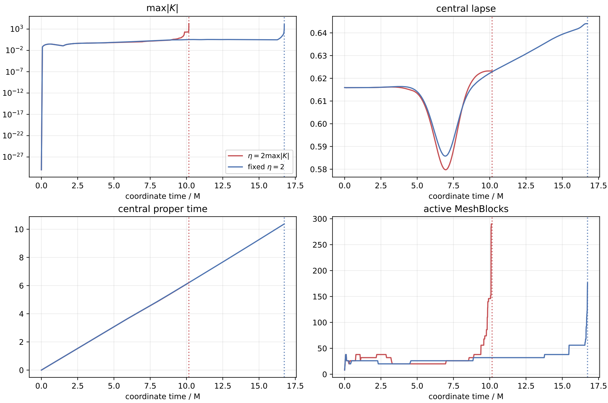
Figure-3 Brill diagnostic: collapse trajectory and AMR
