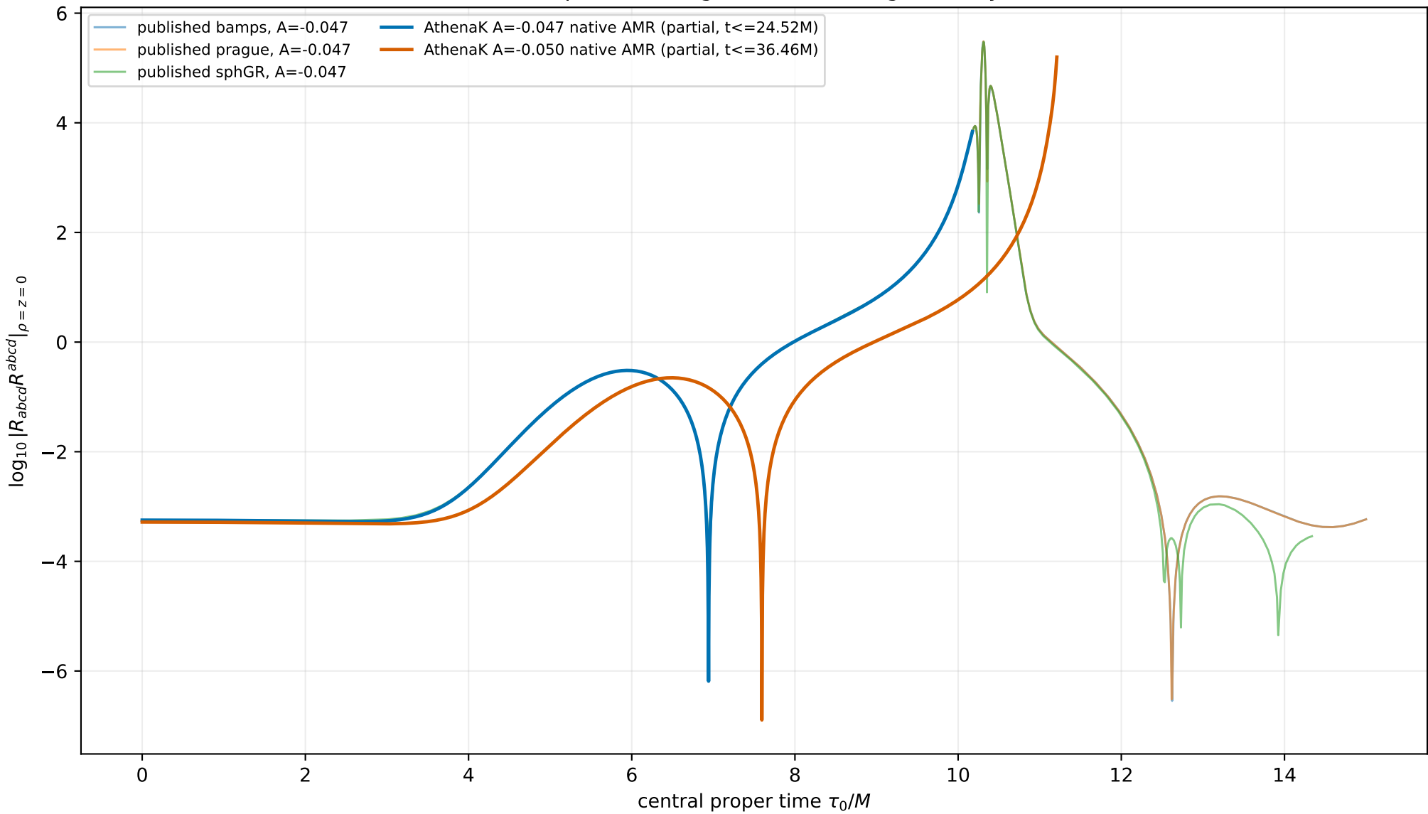
Brill amplitudes: origin curvature (Figure-3 style)
