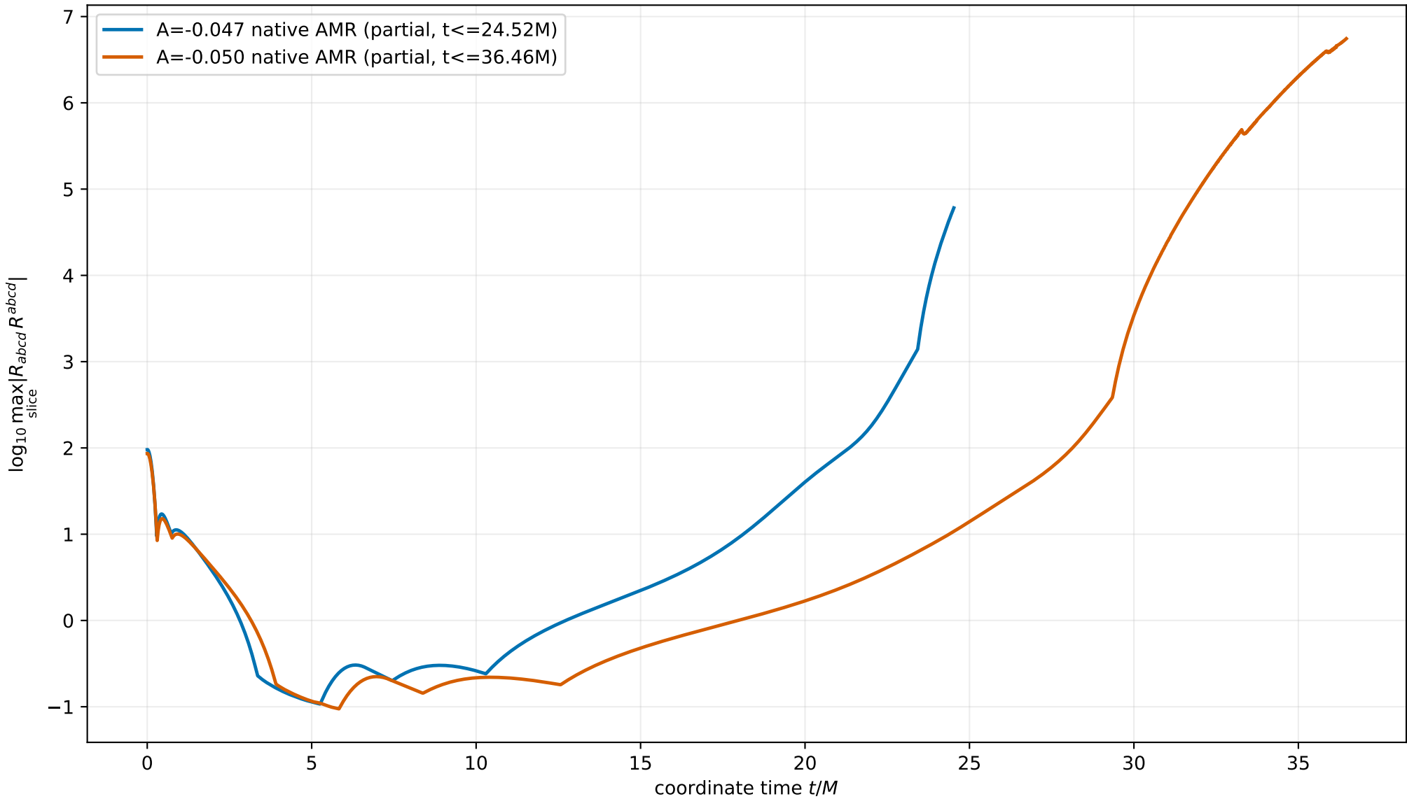
Slice-global maximum Kretschmann scalar
