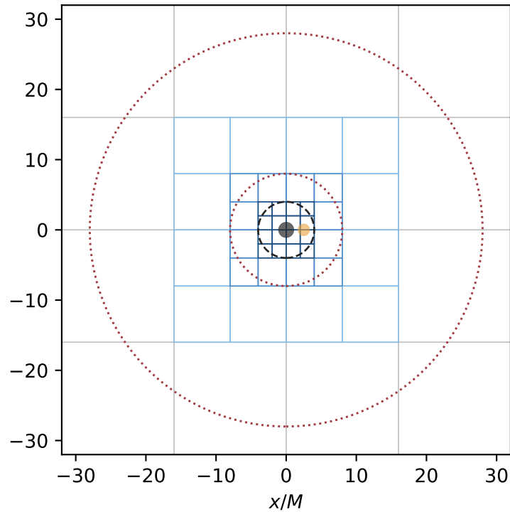
232 blocks; domain \pm 32M
