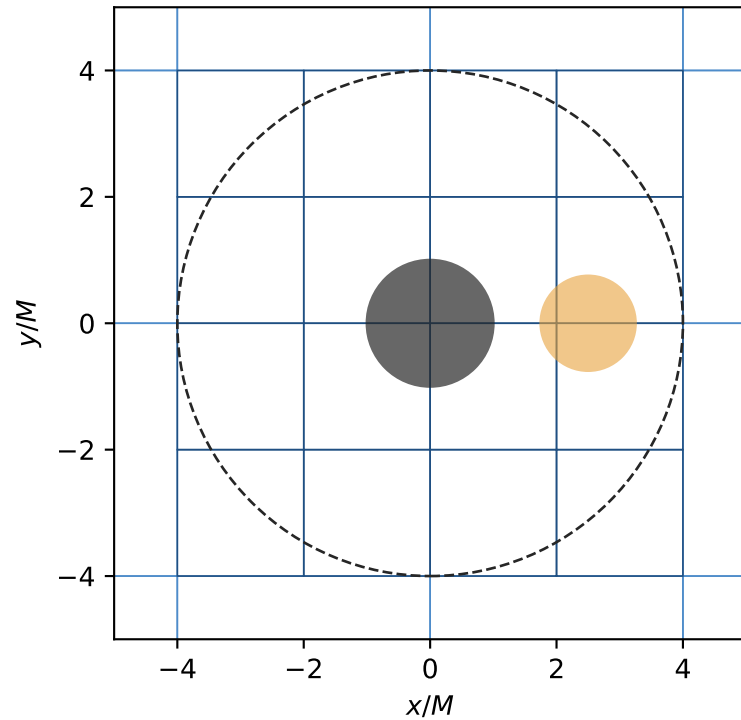
Horizon r=1M ; dx=0.125M
