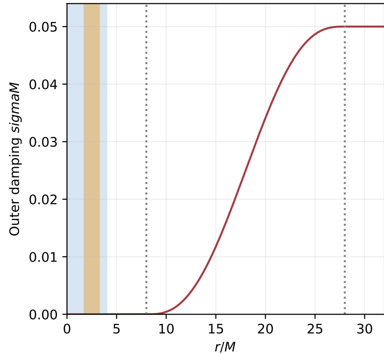
No damping inside r=8M
