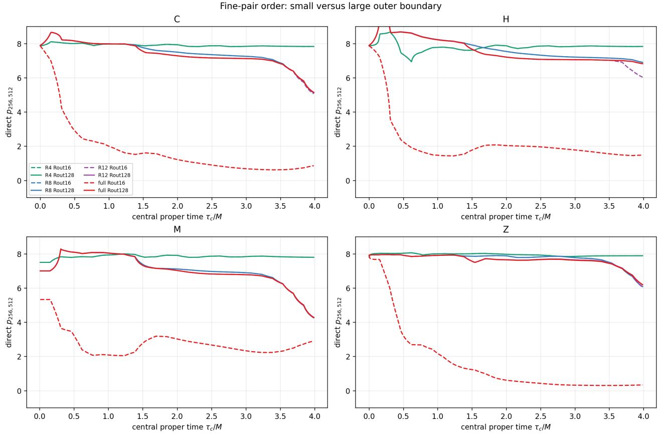
Figure 2: Direct fine-pair order before and after moving the outer boundary.
