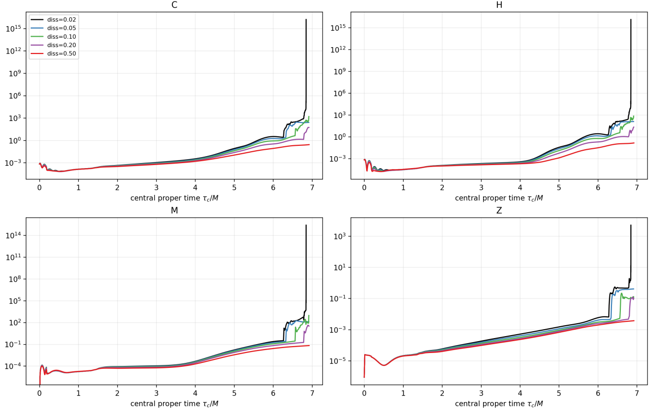
Figure 4: Global constraint inventories versus central proper time.
