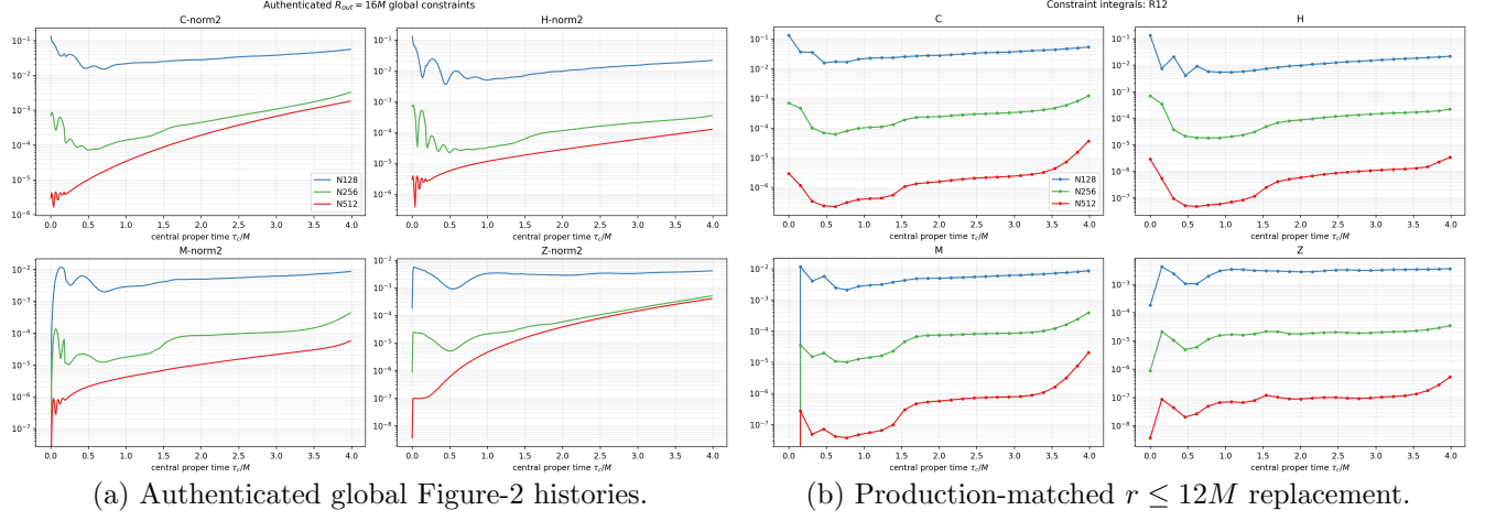
Figure 1: Old global constraint history and the radius-restricted diagnostic shown next to one another.
