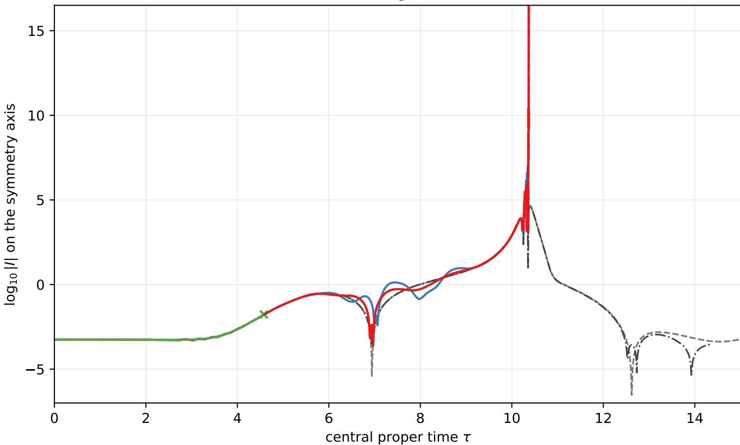
Published Figure-3 scale
