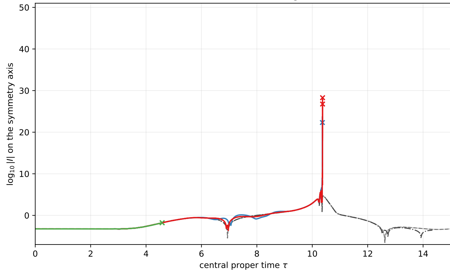
Full finite AthenaK range
