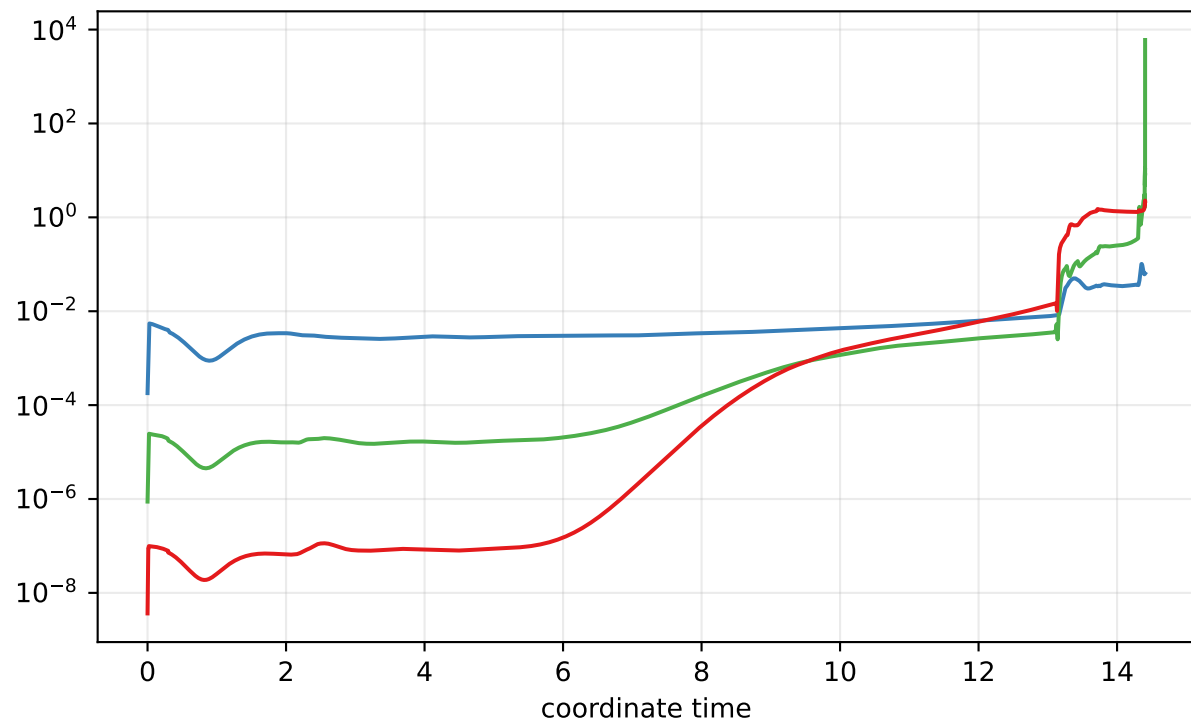
Z-norm2
