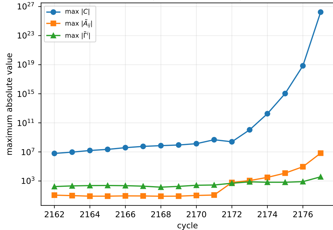
Near-axis puncture-interior growth
