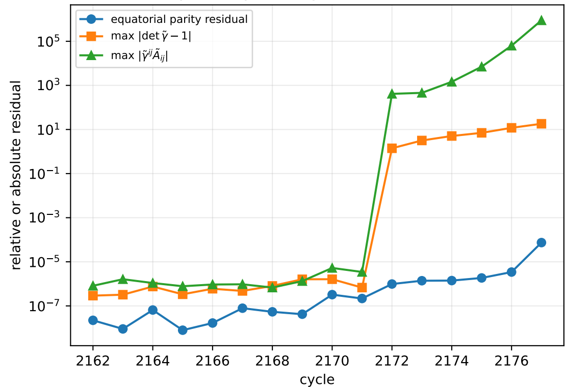
Symmetry and algebraic constraints
