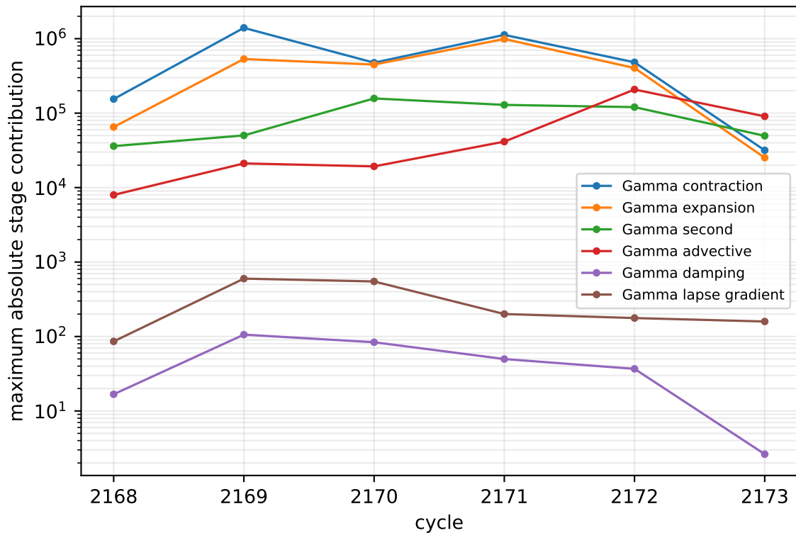
Dominant \tilde{\Gamma}^i RHS pieces
