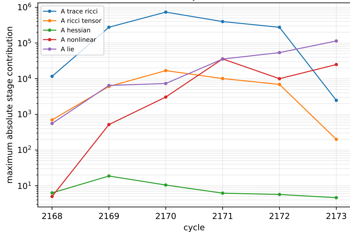
Dominant \tilde{A}_{ij} RHS pieces
