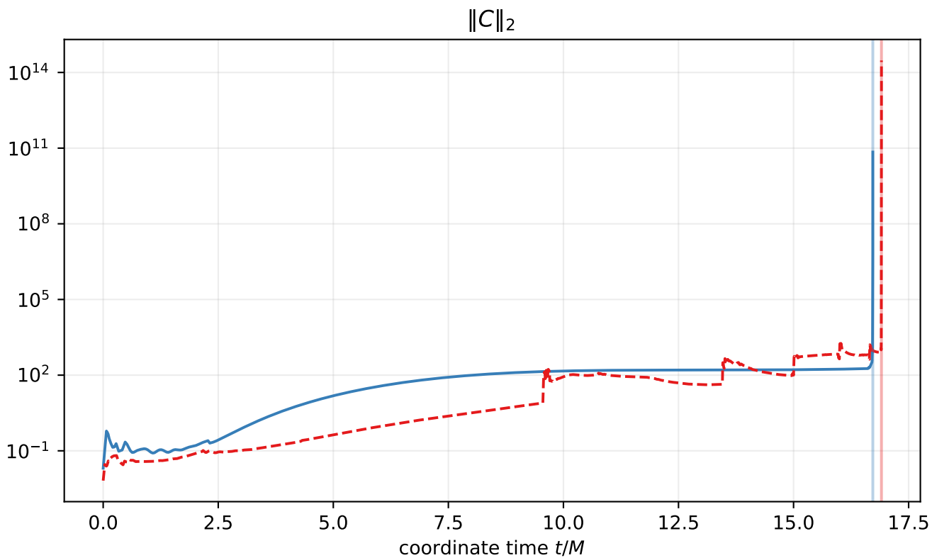
Brill A=-0.047: global constraint histories (vertical lines mark failure)
