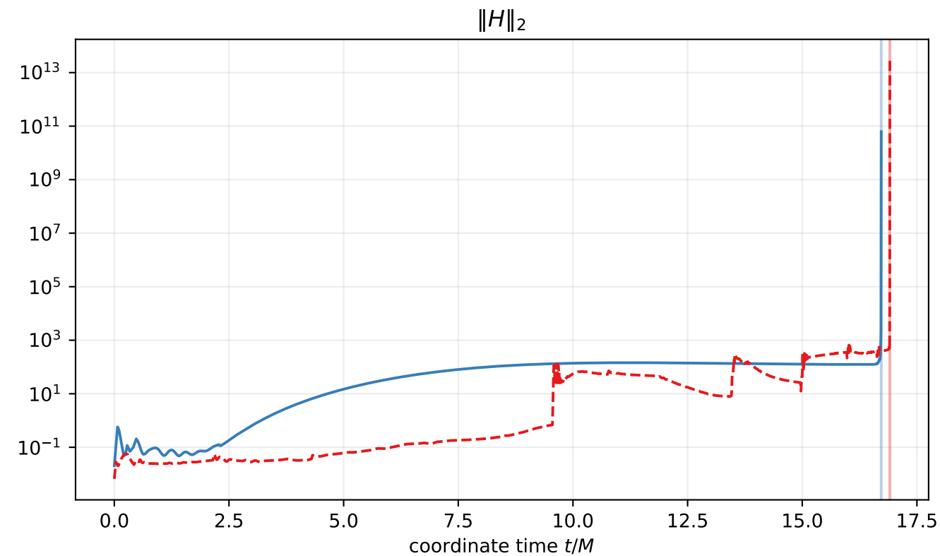
Brill A=-0.047: global constraint histories (vertical lines mark failure)
