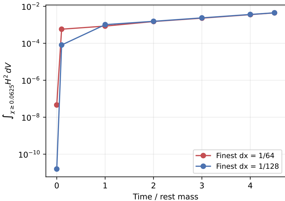
Gamma = 5: partial comparison through 4.5 M An added AMR level refines the central region; the chi mask retains interior points
