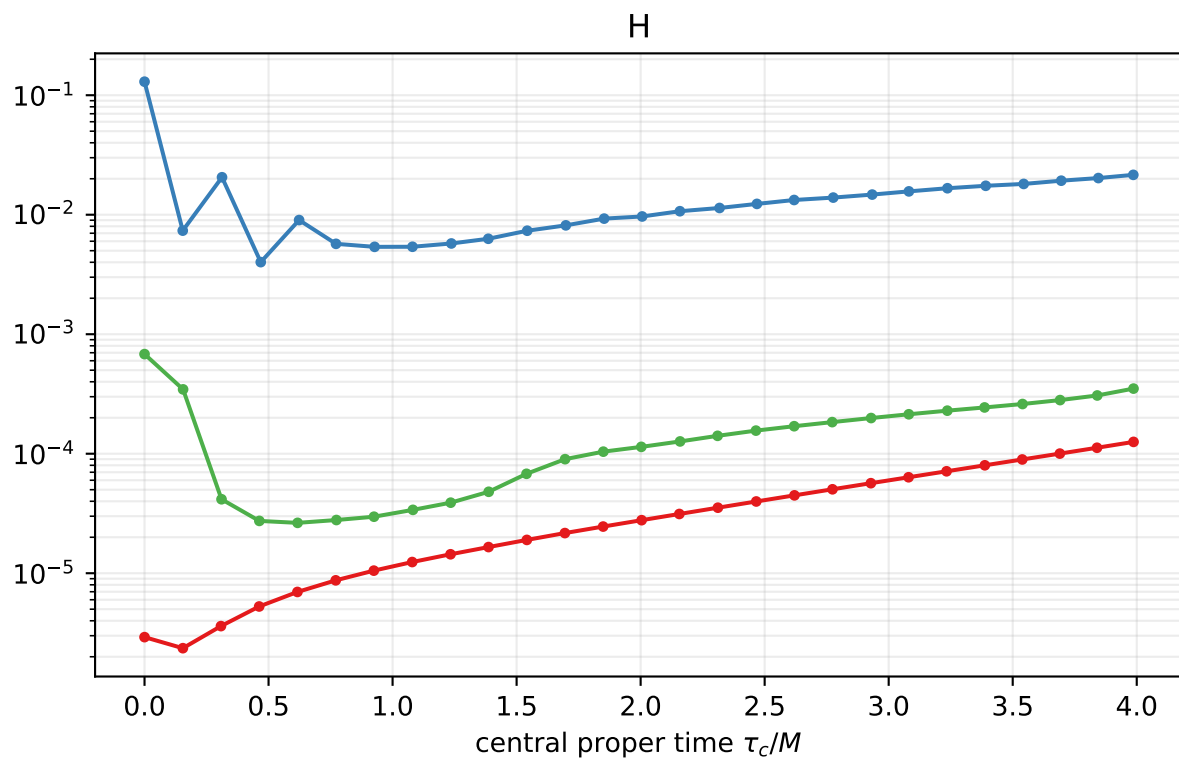
Constraint integrals: full
