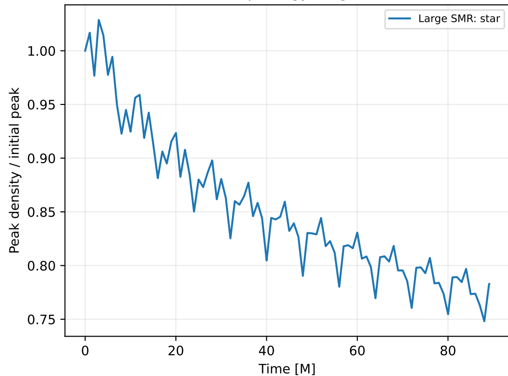
Star morphology diagnostic
