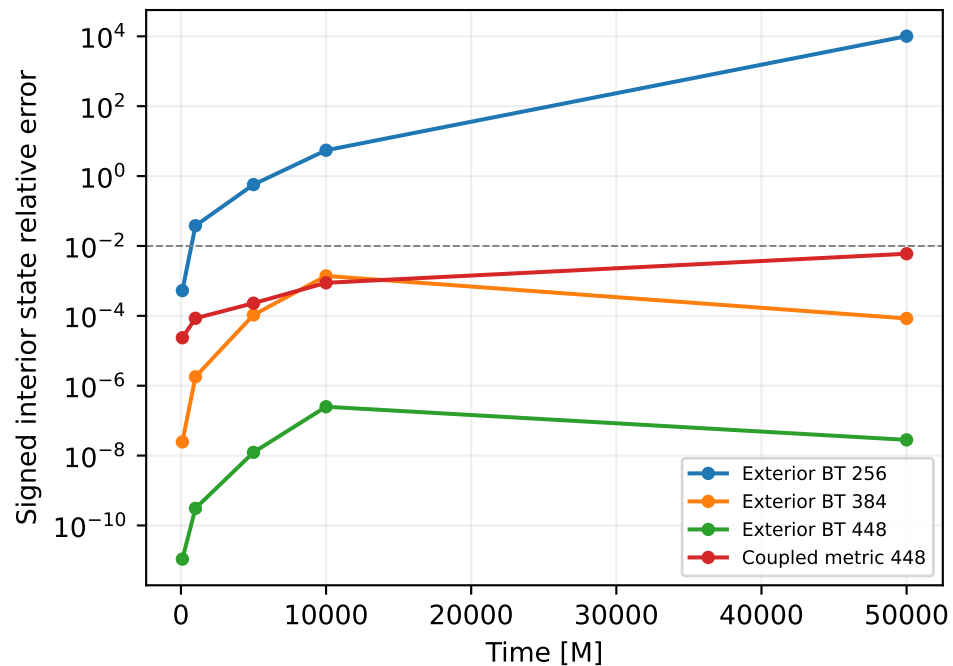
Finite periodic memory fixture · 64 cells / 32 retained · RK3 dt=0.6M
