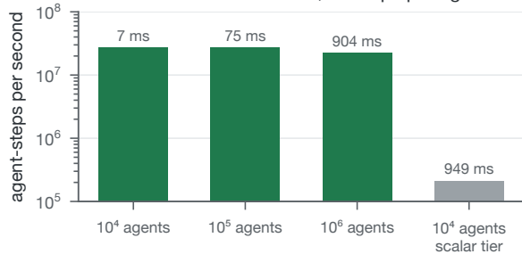
A Execution from the table, 20 steps per agent
