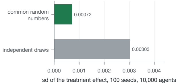
B Common random numbers: variance \div 18
