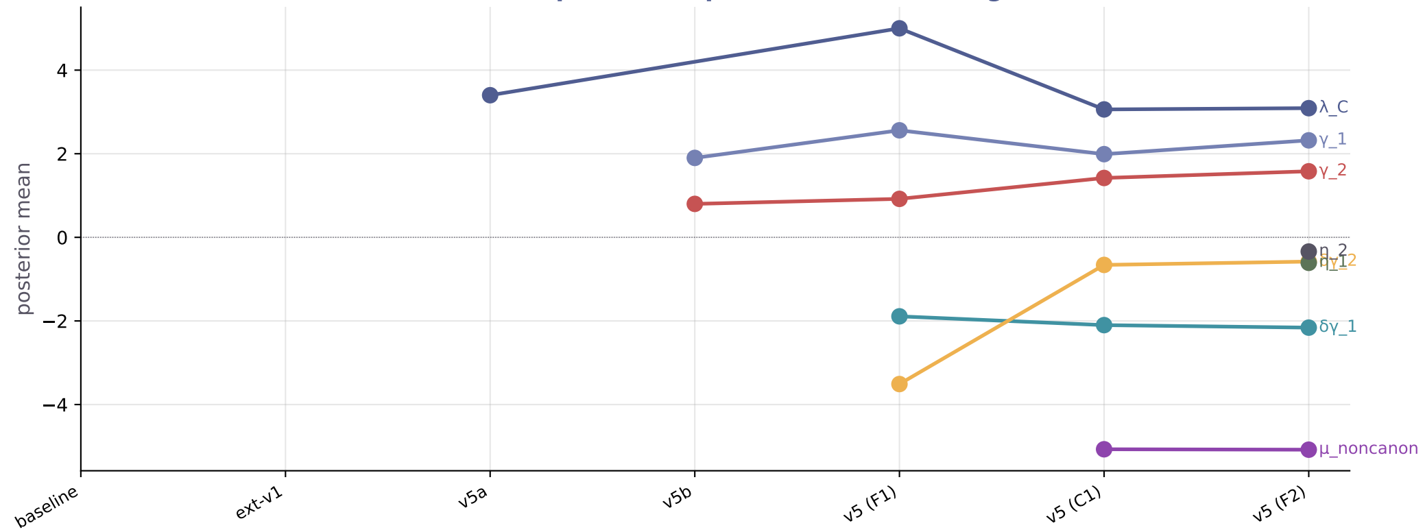
Mechanism parameter posteriors across stages
