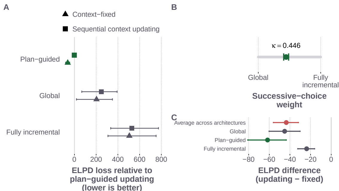
Figure 6: Matched comparisons of production architecture and sequential context updating. Panel A reports predictive loss for all six matched models relative to the plan-guided model with sequential context updating; lower values indicate better leave-one-out prediction. Panel B places the shared successive-choice weight \kappa between the global and fully incremental endpoints. Panel C shows updating-minus-fixed ELPD for each production architecture and their average. Intervals in Panels A and C are 95% credible intervals from the participant-level Bayesian bootstrap; Panel B shows the 95% posterior credible interval for \kappa . The vertical line in Panel C marks zero.
