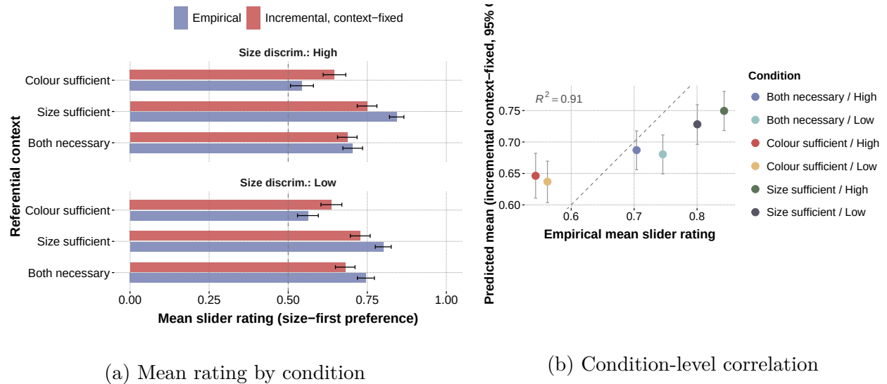
Figure 6 (a) Mean rating by condition (b) Condition-level correlation Posterior-predictive fit of the heldout-best incremental context-fixed slider model. (a) Observed mean slider ratings and posterior-predictive model means by referential context \times size discriminability; dashed line marks 0.5 (no preference), error bars are 95% confidence and posterior-predictive intervals. (b) Observed vs. predicted condition means; dashed line is identity.
