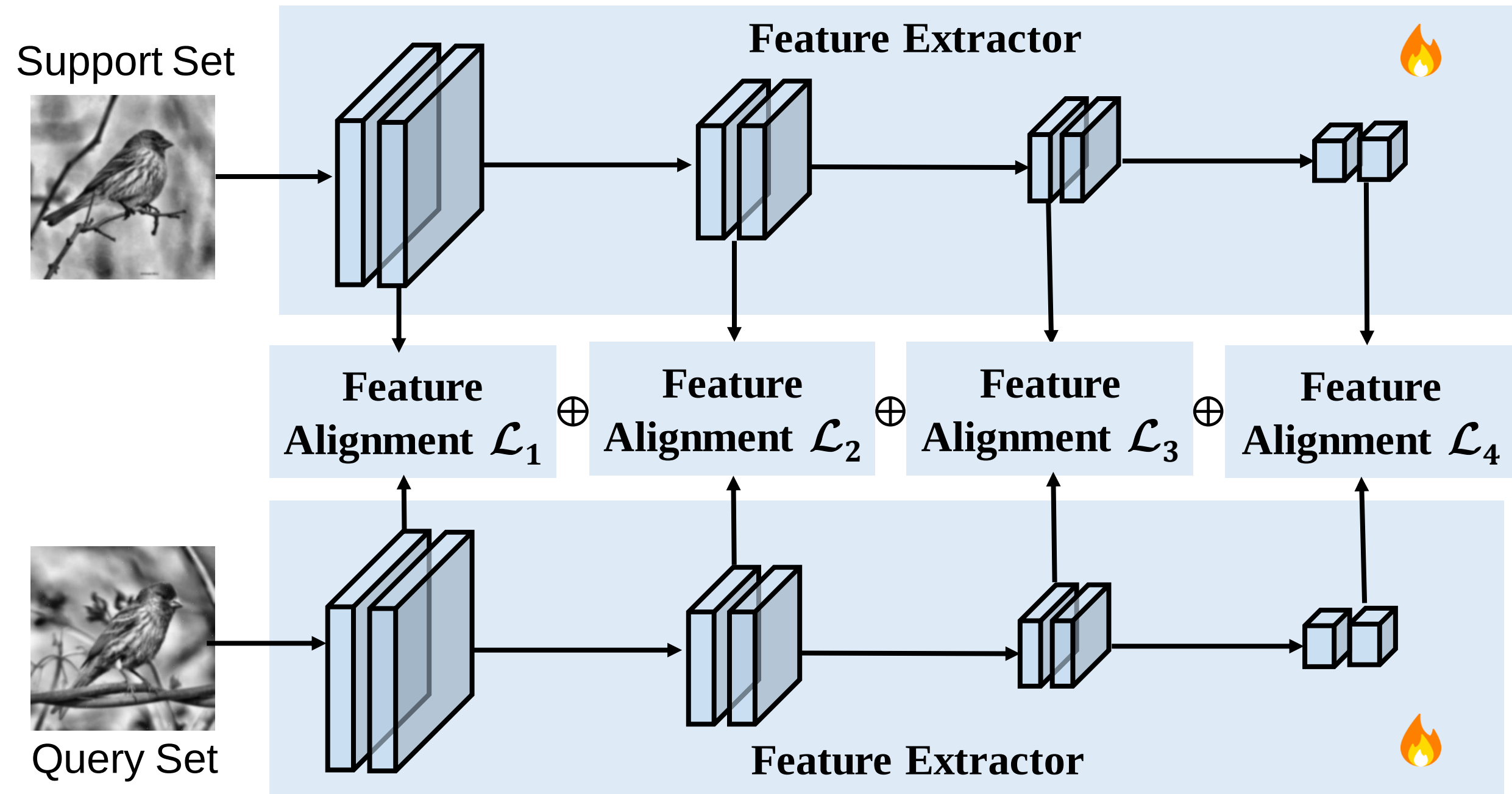
(b) Multi-Branch Meta-Training Feature Alignment
