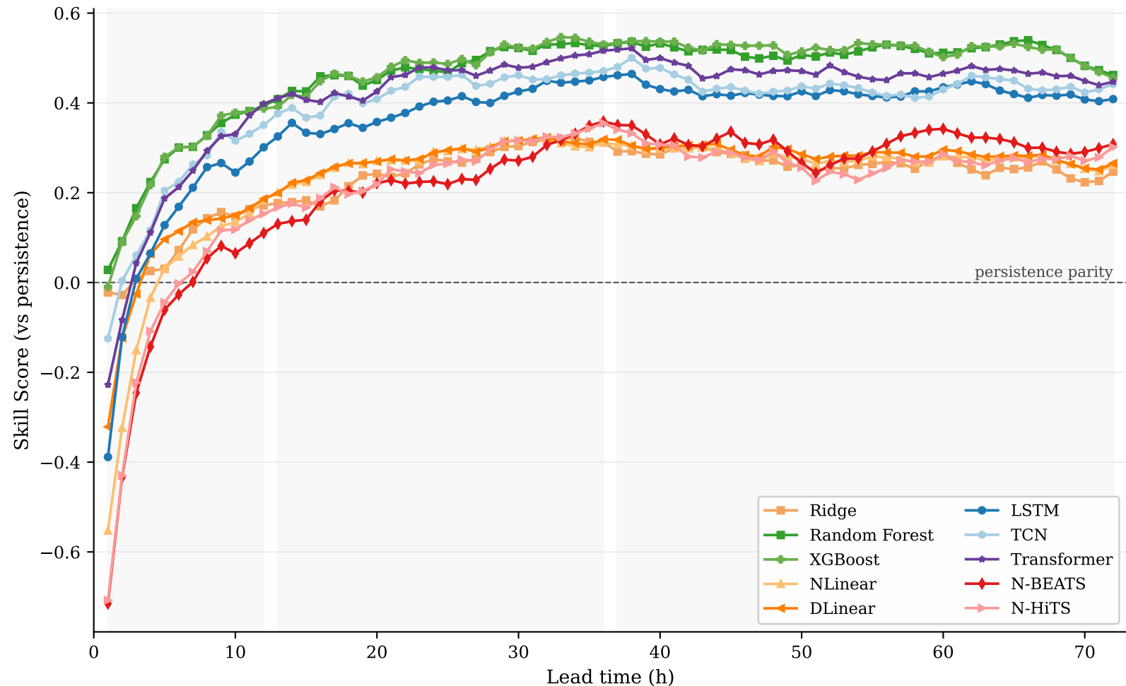
Nz Farm4 — Skill Score vs Forecast Horizon
