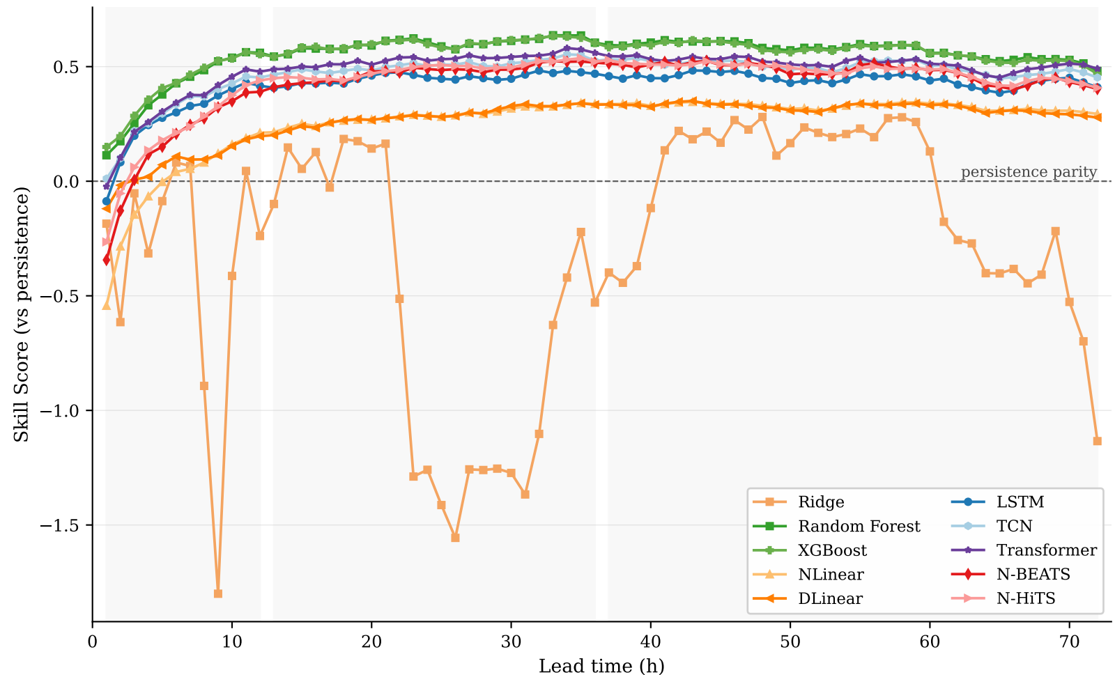
Nz Farm11 — Skill Score vs Forecast Horizon
