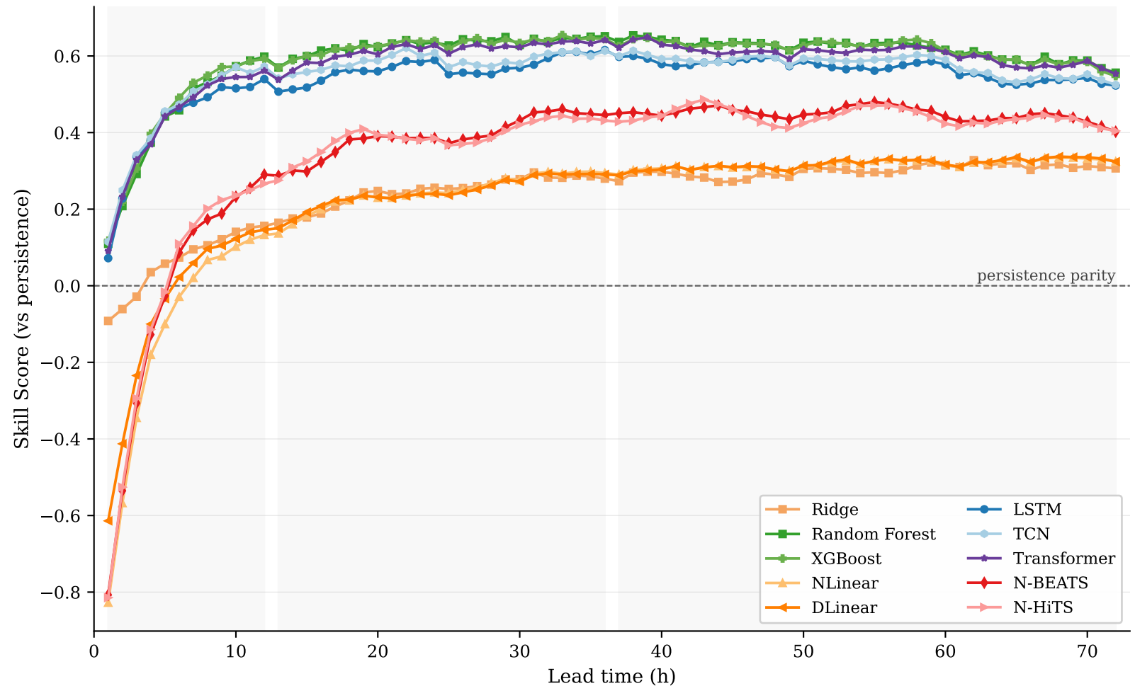
Kelmarsh — Skill Score vs Forecast Horizon
