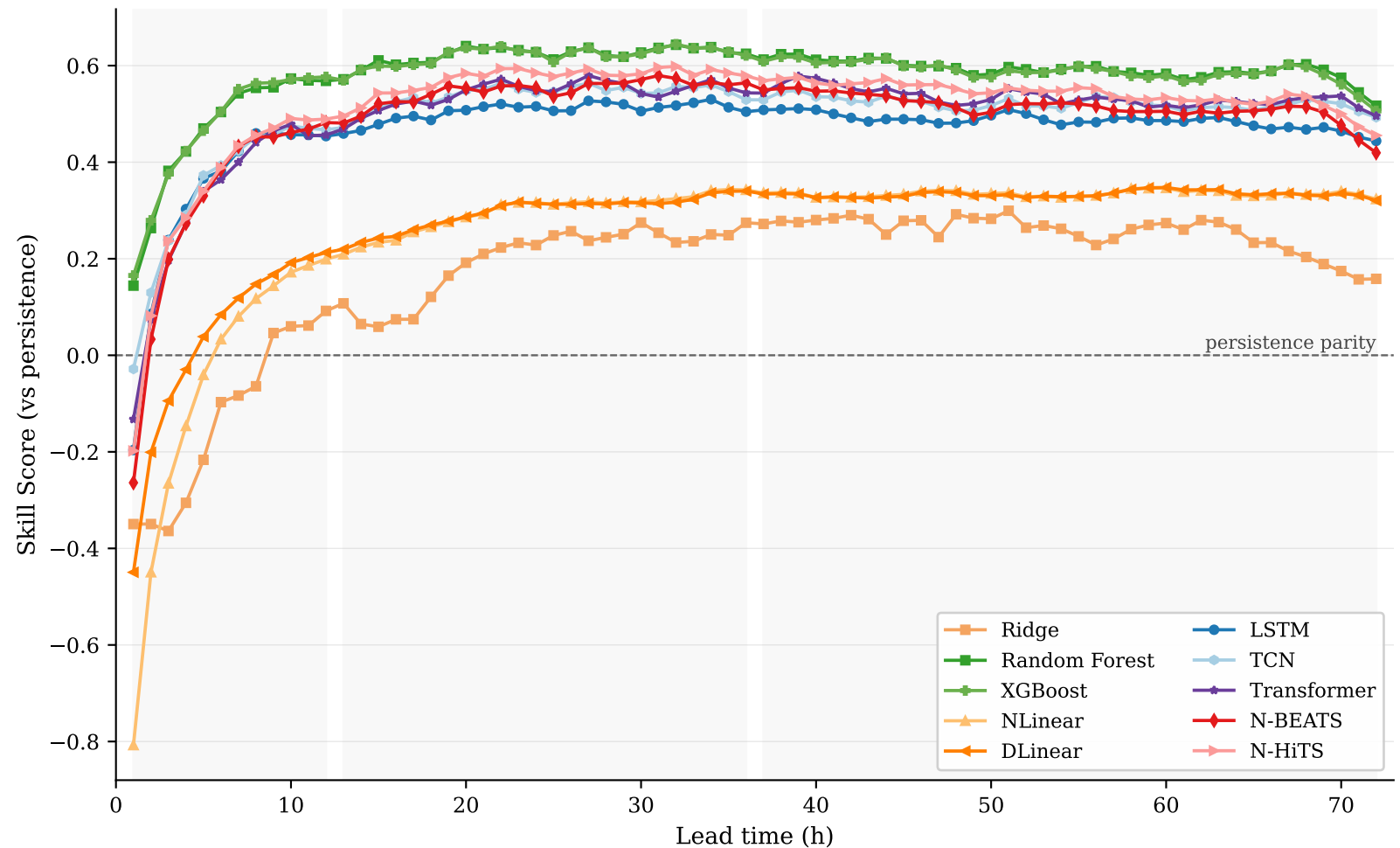
Nz Farm12 — Skill Score vs Forecast Horizon
