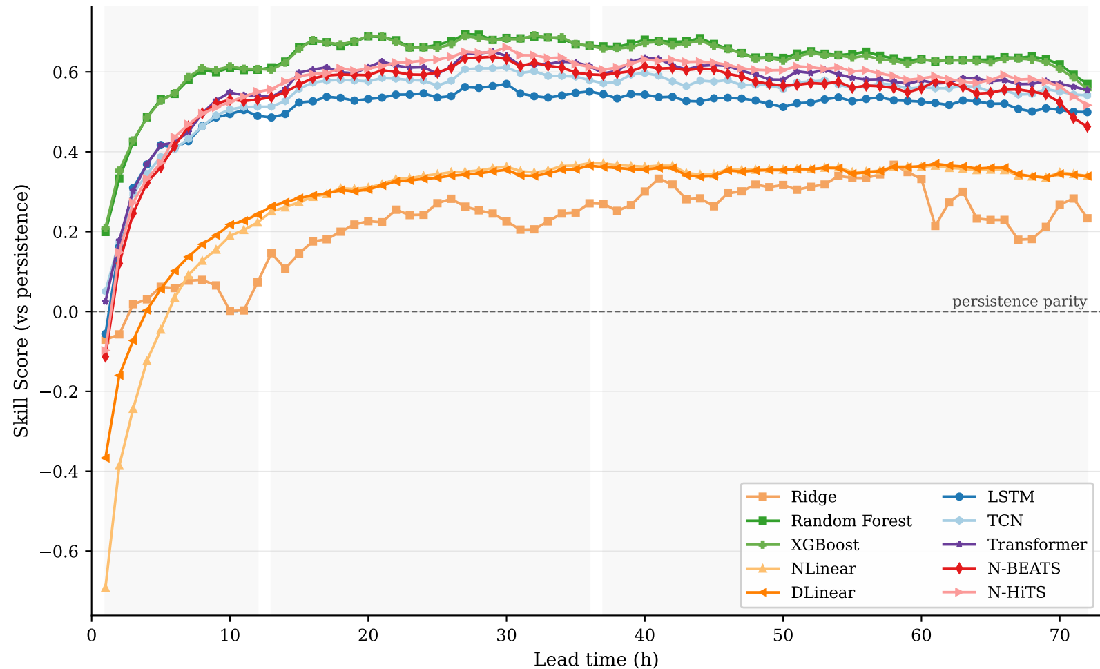
Nz Farm5 — Skill Score vs Forecast Horizon
