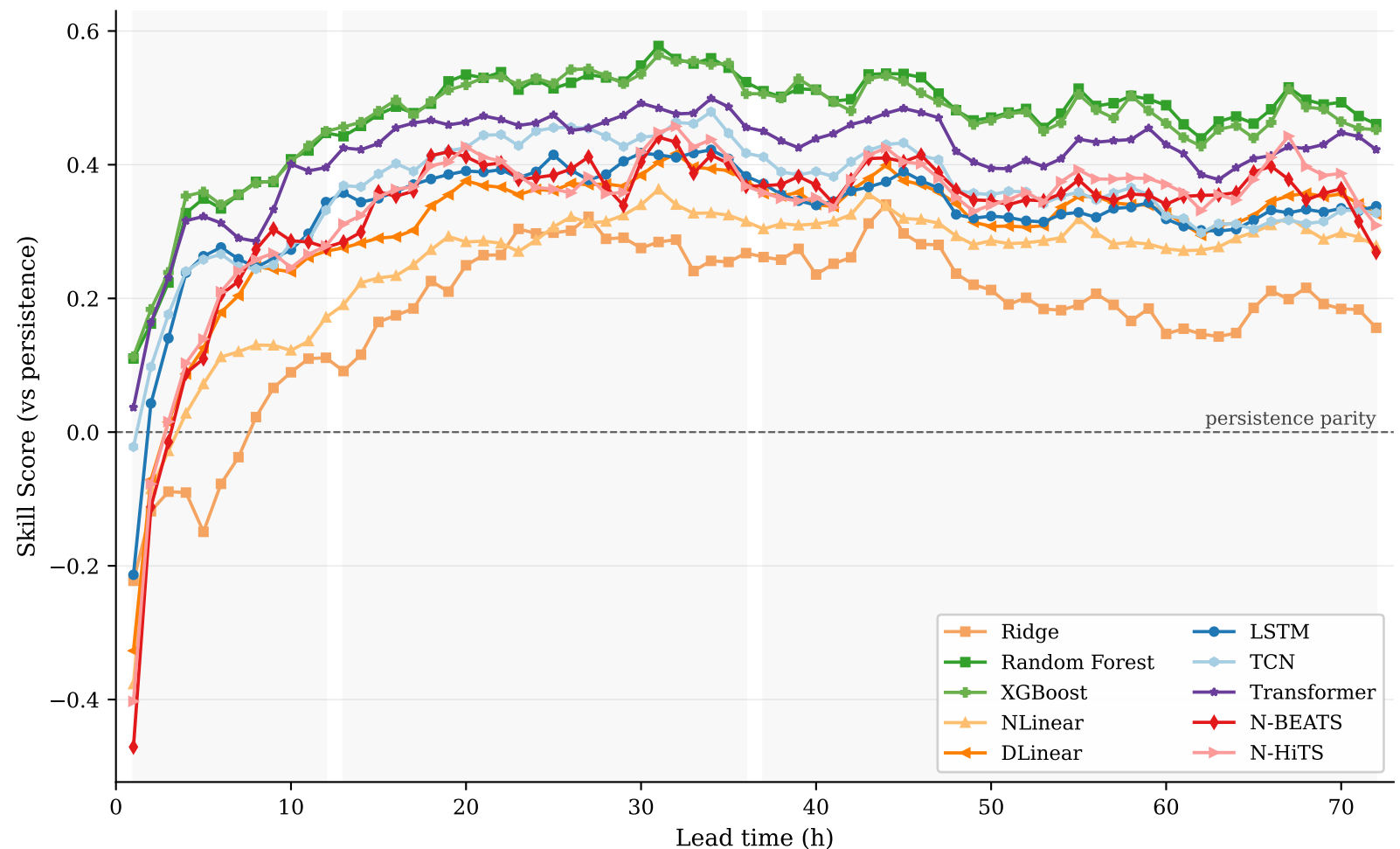
Nz Farm13 — Skill Score vs Forecast Horizon
