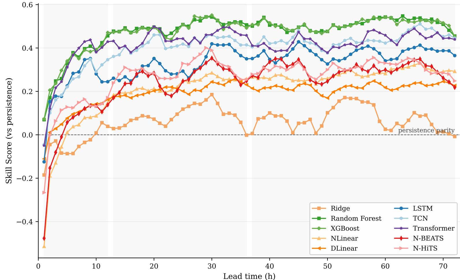
Nz Farm9 — Skill Score vs Forecast Horizon
