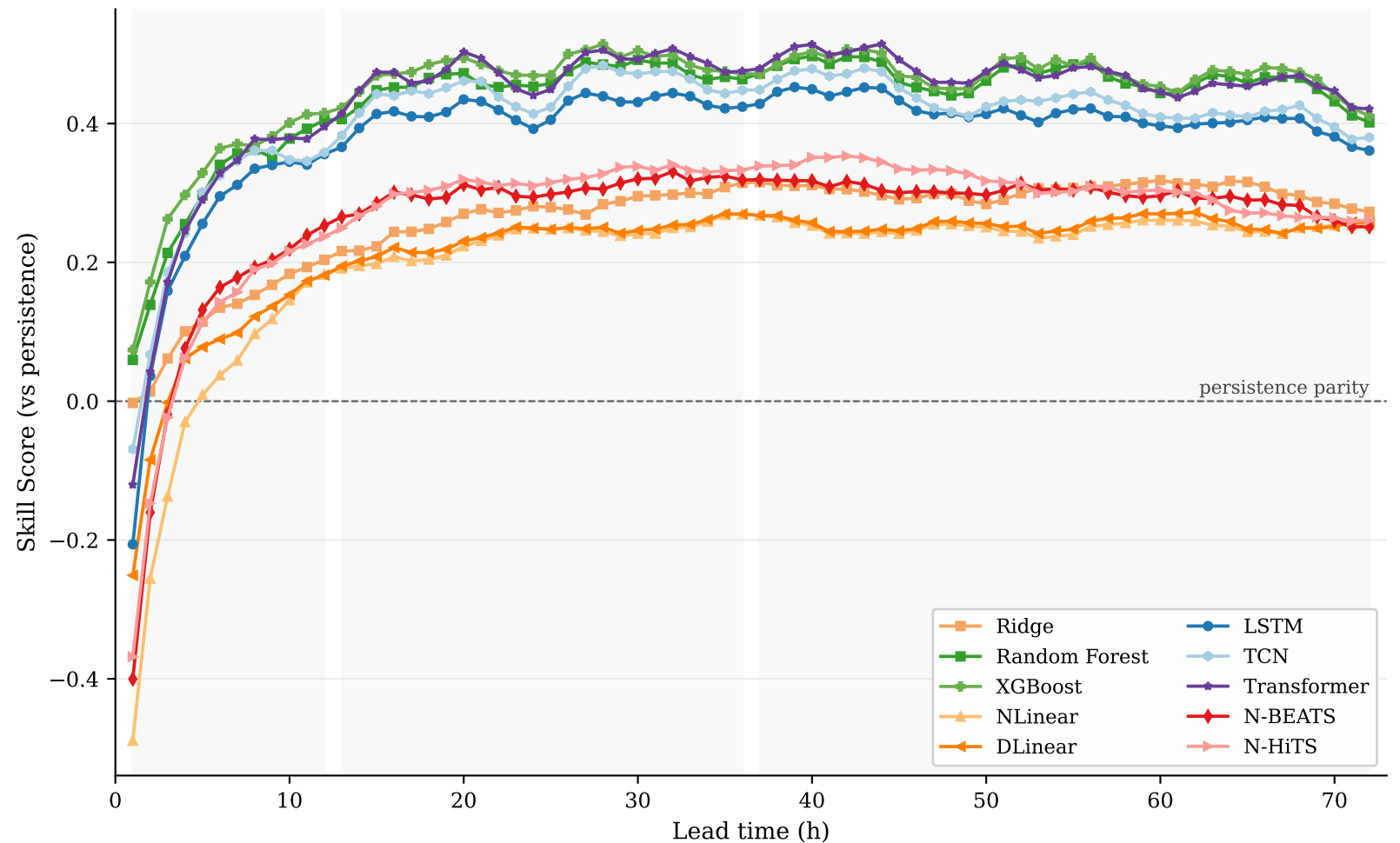
Nz Farm10 — Skill Score vs Forecast Horizon
