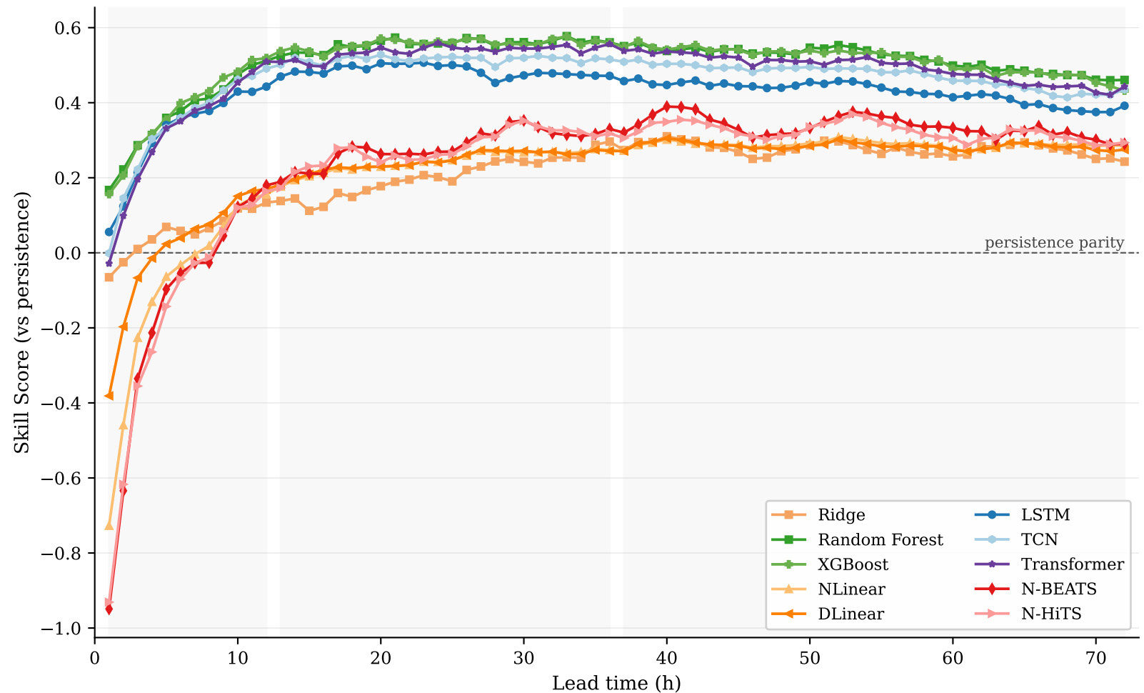
Penmanshiel — Skill Score vs Forecast Horizon
