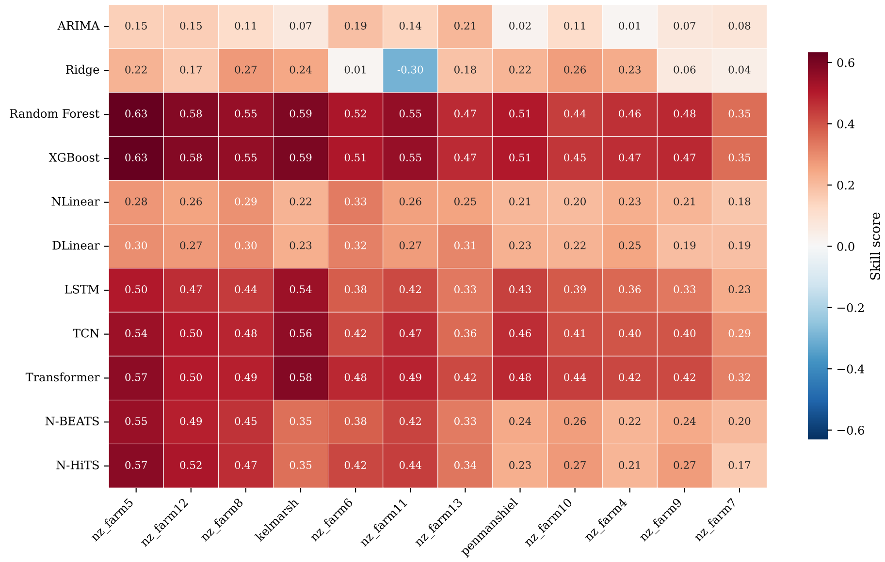
Skill Score per (Model, Farm) — averaged over all 72 lead times
