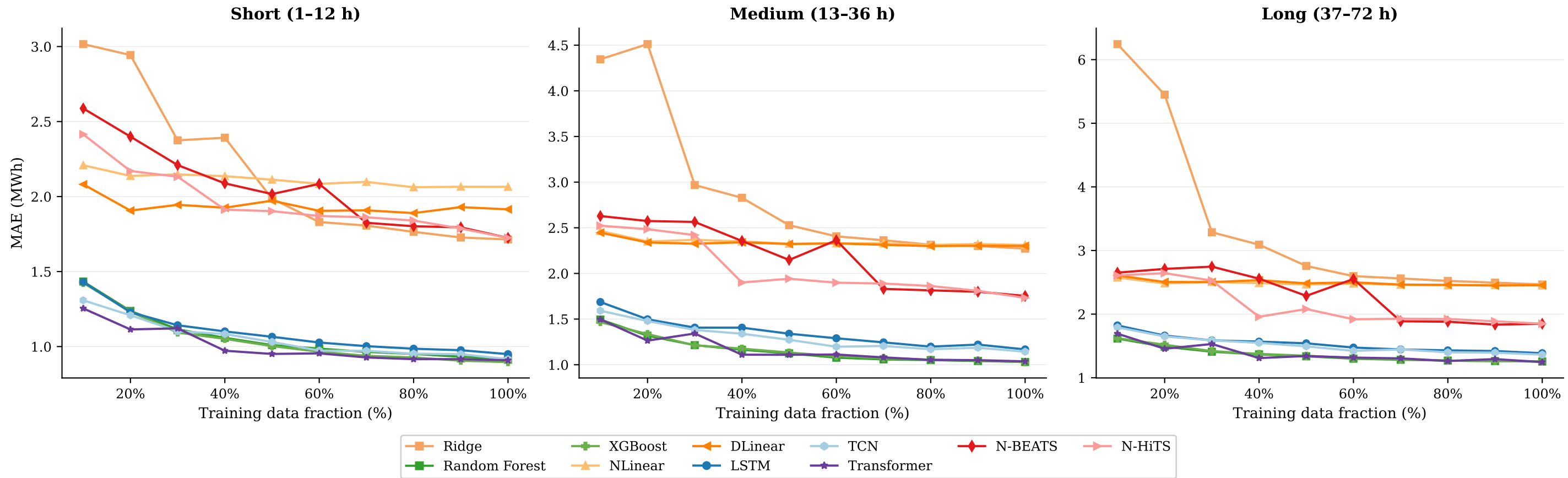
Data Scaling on Kelmarsch — MAE vs Training-Set Size by Horizon Bin
