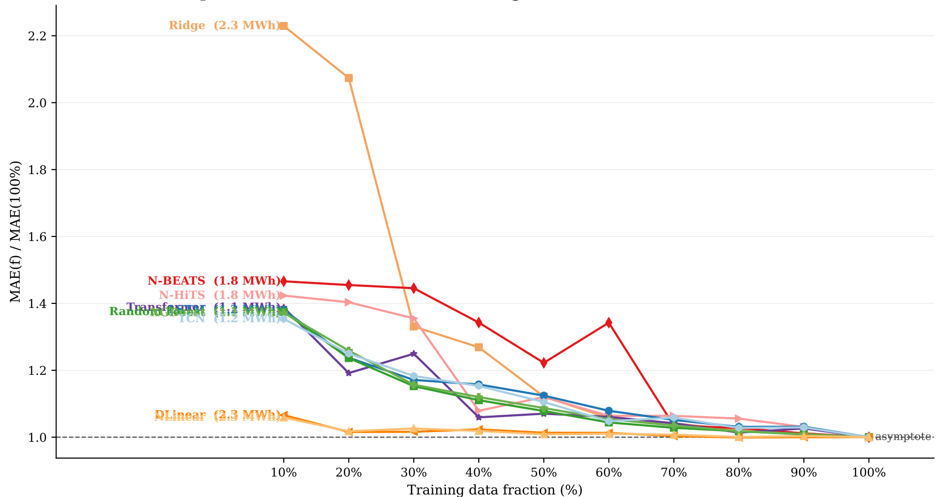
Sample Efficiency — Normalized Learning Curves on Kelmarsh (steeper curves = more sensitive to training-set size; MAE@100% shown in MWh)
