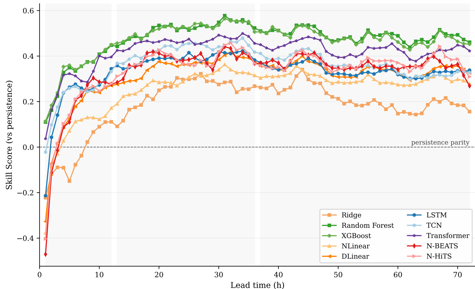
Nz Farm13 — Skill Score vs Forecast Horizon
