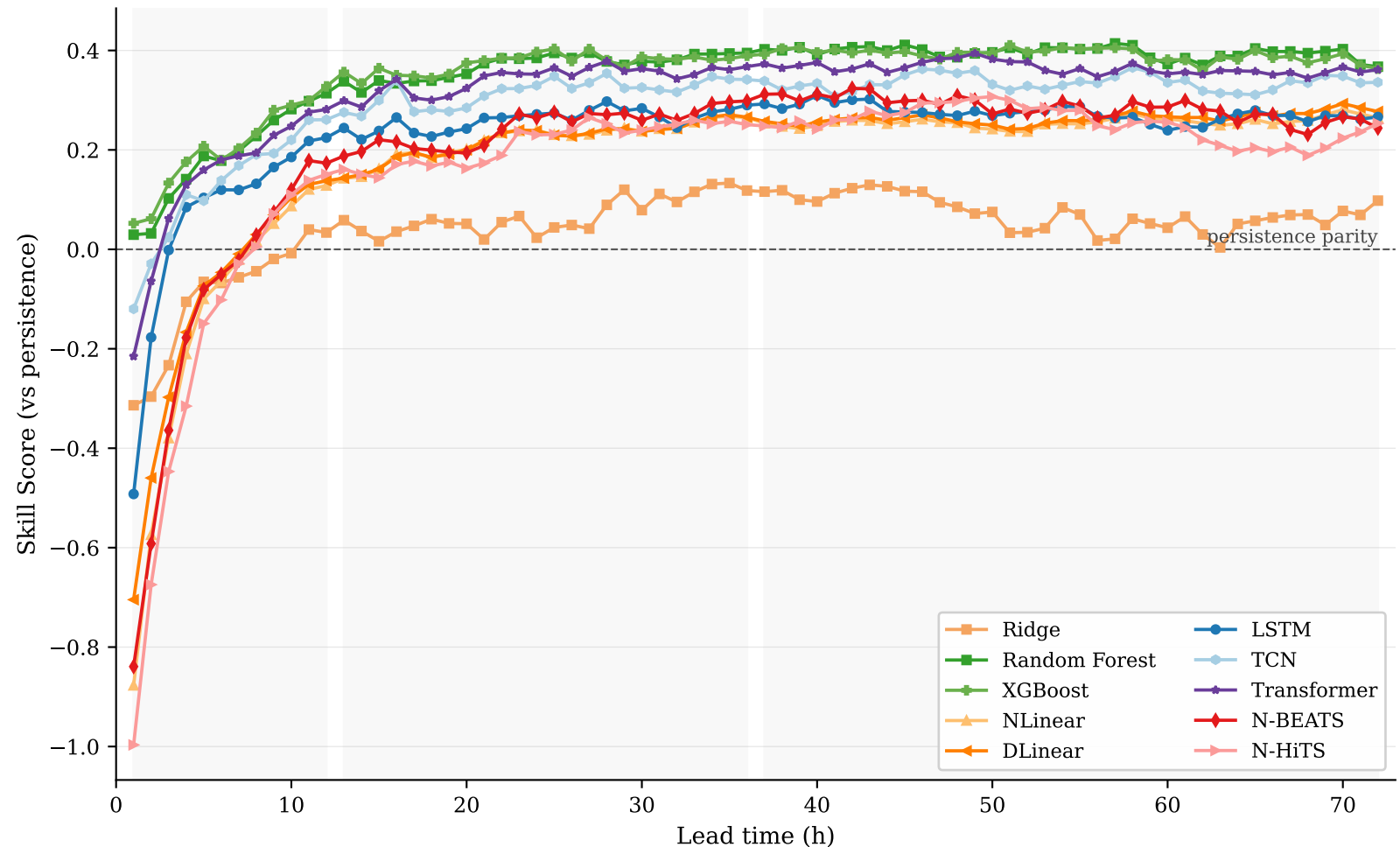
Nz Farm7 — Skill Score vs Forecast Horizon
