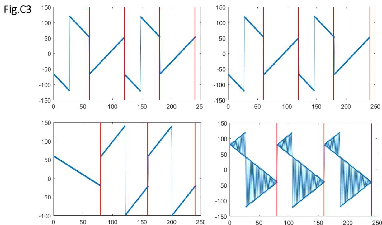
Fig.C3. Phase encoding order for 'faisé' (left) and 'centric' for segmented acquisition with 4(top) and 3(bottom) segments. For an even number of segments, both phase encoding schemes yield identical phase encoding ordering, but they differ for odd number of segments.
