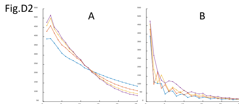
Fig.D2 Signal decay for gray matter under CPMG(A) and CP(B) conditions for gray matter and refocusing flip angles 60(blue), 90(red), 120 (yellow), and 150(magenta) degrees.
