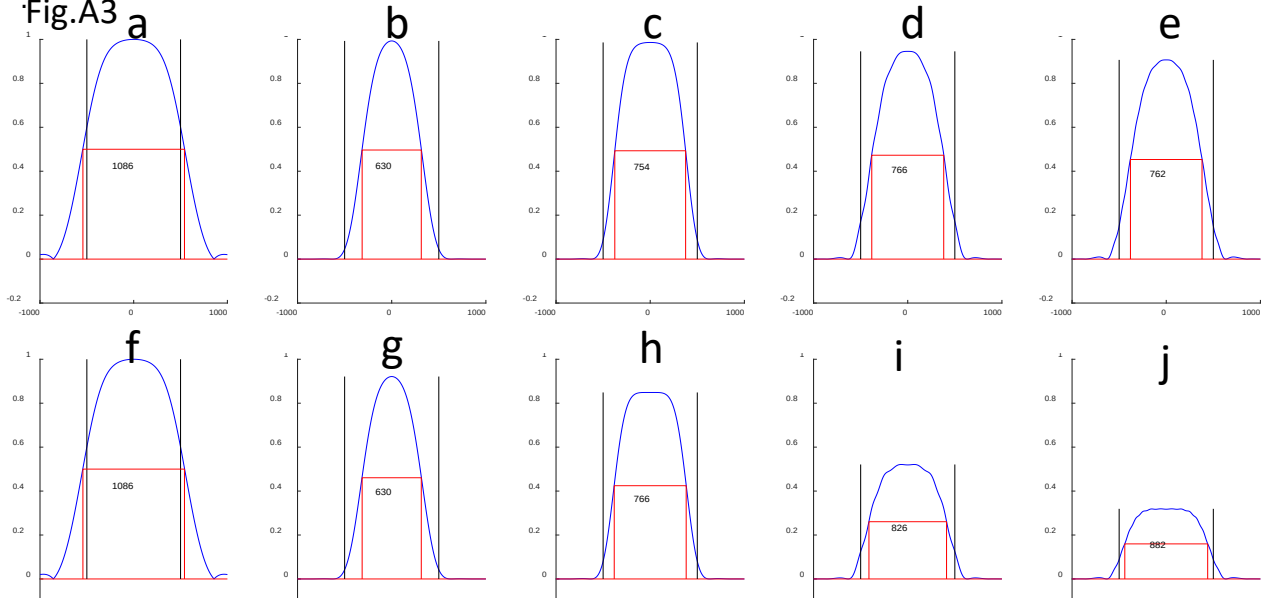
Fig.A3 response profile of the excitation pulse (a,f) and of the first(b,g), 2 nd (c,h), 8 th (d, i) and 14 th (e,j) echo for nominal refocusing flip angle 180^\circ and T1/T2 = 3.65/1.43 ms (CSF, a-e) and 907/92 ms(gray matter, f-j). Excitation pulse duration/ tBwP = 4 ms/4, refocusing pulse 2 ms/2;
