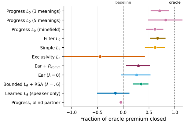
Figure 1: The results on one axis: fraction of each environment’s oracle premium closed (dots; bootstrap 95% CIs over seeds). Bounded motion-grounded listeners transfer across environments; the saturated learned listener sits at or below zero; the blind control (scaled by its own premium) sits at zero.
