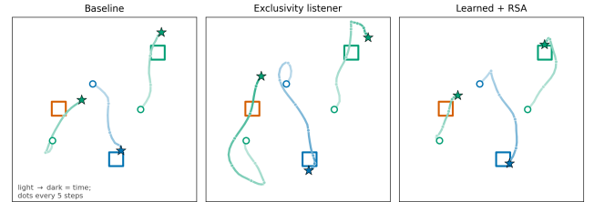
Figure 9: A converged evaluation episode under three conditions. Squares are landmarks (color = category); trajectories are colored by the agent’s private preference and darken with time. The exclusivity-listener agents sweep the arena and settle off-landmark—costly motion signaling nothing; the learned-pragmatic agents take direct, mutually distinct paths.
