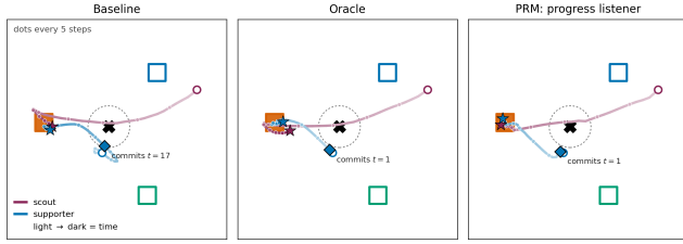
Figure 7: One Environment A evaluation episode under three conditions (selected from 60 candidates to maximize the baseline-vs-recipe commitment-time difference; statistics are in Table 1). Squares are sites (target filled); cross and dashed circle mark the pickup waypoint; trajectories darken with time; diamond = the supporter’s commitment moment. The baseline supporter commits at t=17 ; the pragmatically rewarded supporter commits at t=1 , matching the oracle.
