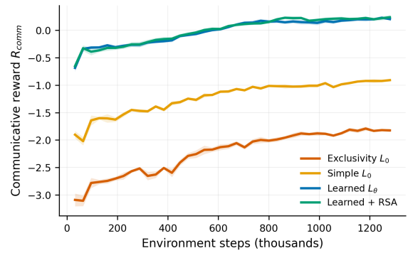
Figure 8: Achieved communicative reward R_{comm} over training (each condition under its own listener; 0 = uninformative). Calibration levels separate: learned listeners cross into positive information gain; the exclusivity listener never leaves negative territory—the miscalibration certificate.
