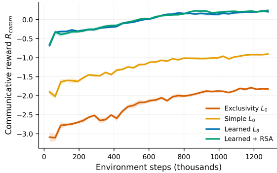
Figure 8: Achieved communicative reward R_{\text{comm}} over training (each condition under its own listener; 0 = uninformative). Calibration levels separate: learned listeners cross into positive information gain; the exclusivity listener never leaves negative territory—the miscalibration certificate.
