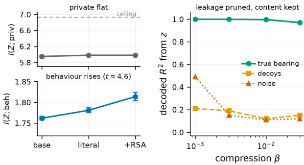
Figure 6: Two separable dials in the self-assigned regime. Left (each strip on its own scale): the legibility reward raises I(Z; \text{behaviour}) ( t \approx 4.6 ) while I(Z; \text{private}) stays flat across conditions, well below the K=1023 critic ceiling. Right: stronger compression ( \beta ) prunes decoded noise leakage from z while the true bearing stays fully decodable.
