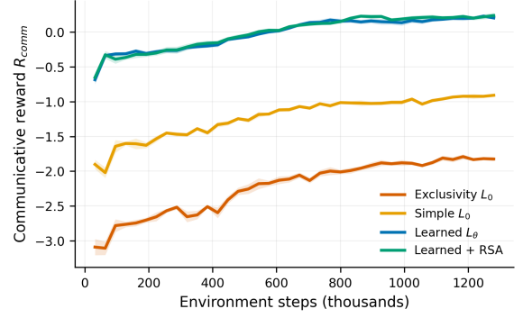
Figure 8: Achieved communicative reward R_{\text{comm}} over training (each condition under its own listener; 0 = uninformative). Calibration levels separate: learned listeners cross into positive information gain; the exclusivity listener never leaves negative territory—the miscalibration certificate.
