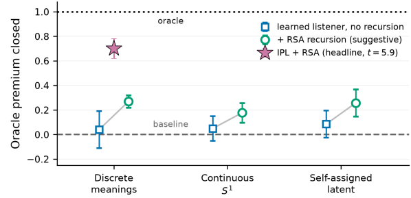
Figure 5: The meaning-space axis. In each regime the learned listener without recursion sits near the baseline; one RSA step lifts it by a similar fraction everywhere, but only the inverse-planning listener in the discrete regime clears the t \geq 4 headline bar (filled star). The hand-crafted listeners (Table 1, 60–82%) are a separate family, omitted here to isolate the recursion’s effect on the learned one. Whiskers are \pm 1 s.e.m. as a fraction of each regime’s oracle premium.
