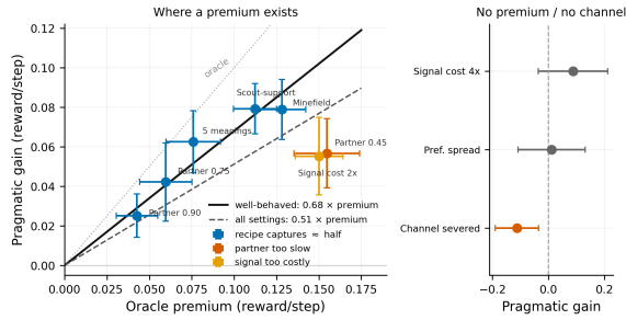
Figure 3: The boundary map. Left: across every setting with a resolvable premium, gain scales with premium (solid: well-behaved fit 0.68\times ; dashed: all settings 0.51\times ; dotted: oracle). Settings where the partner is too slow or signaling too costly fall below despite large premiums. Right: no premium / no channel. Left bars \pm 1 s.e.m., right bars 95% CIs.
