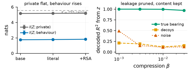
Figure 6: Two separable dials in the self-assigned regime. Left: the legibility reward raises I(Z; \text{behavior}) across conditions while I(Z; \text{private}) stays flat below the critic ceiling. Right: stronger compression ( \beta ) prunes decoded noise leakage from z while the true bearing remains fully decodable.
