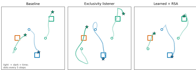
Figure 7: A converged evaluation episode under three conditions. Squares are landmarks (color = category); trajectories are colored by the agent’s private preference and darken with time. The exclusivity-listener agents sweep the arena and settle off-landmark—costly motion signaling nothing; the learned-pragmatic agents take direct, mutually distinct paths.
