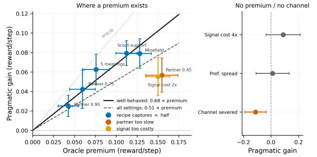
Figure 4: The boundary map. Left: across every setting with a resolvable premium, gain scales with premium (solid: well-behaved fit 0.68\times ; dashed: all settings 0.51\times ; dotted: oracle). Settings where the partner is too slow or signaling too costly fall below despite large premiums. Right: no premium / no channel. Left bars \pm 1 s.e.m., right bars 95% CIs.
