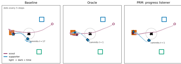
Figure 3: One evaluation episode under three conditions (selected from 60 candidates to maximize the baseline-vs-recipe commitment-time difference; statistics are in Table 1). Squares are sites (target filled); cross and dashed circle mark the pickup waypoint; trajectories darken with time; diamond = the supporter’s commitment moment. The baseline supporter hesitates and commits at t=17 ; the pragmatically rewarded supporter commits at t=1 , matching the oracle.
