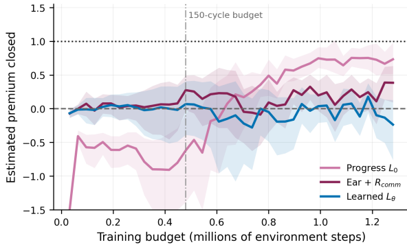
Figure 5: The pre-convergence hazard: estimated fraction of the premium closed vs. the training budget at which the comparison is made (bootstrap 95% bands, 10 seeds). The ordering stabilizes only past \sim 1\text{M} steps.
