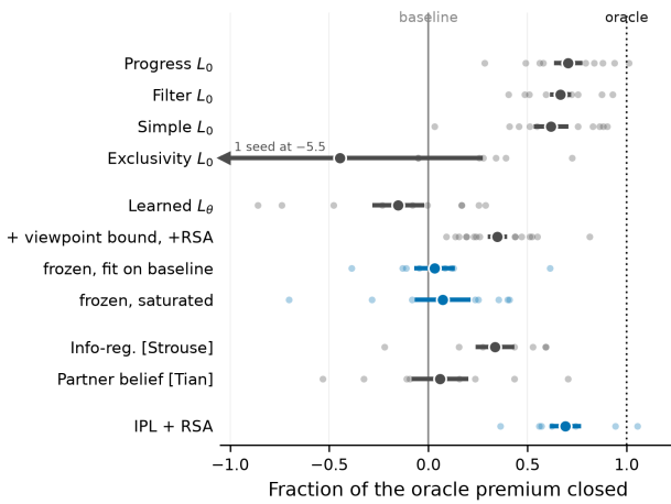
Figure 3: Which listener pays, in Environment A. Dots are seeds, bar \pm 1 s.e.m., marker the mean; blue marks the rows the argument turns on. Exclusivity is bimodal rather than merely uncertain: seven seeds at .3-.6 , one off-scale. Exact values in Table 1.
