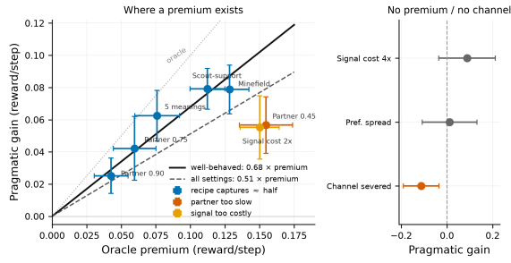
Figure 2: The boundary map. Left: where the premium is resolvable, gain scales with it (solid: well-behaved fit 0.68\times ; dashed: all settings 0.51\times ; dotted: oracle); too-slow partners and too-costly signaling fall below despite large premiums. Right: no premium / no channel. Left bars \pm 1 s.e.m., right bars 95% CIs.
