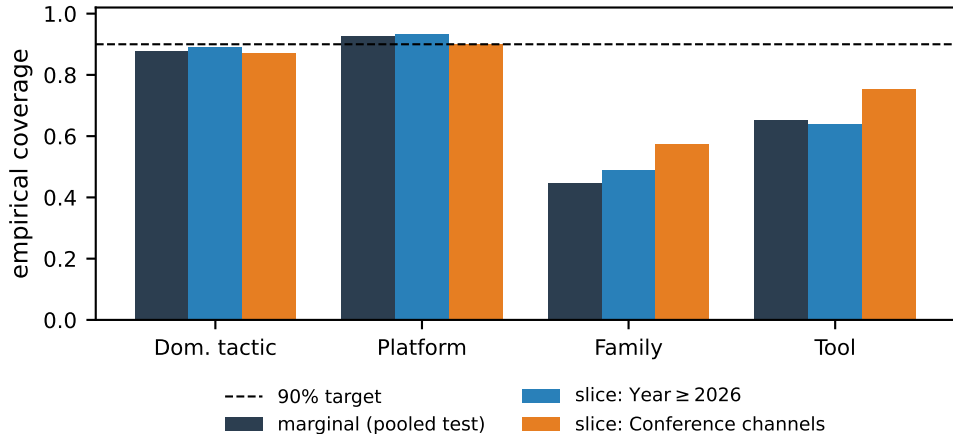
Split-conformal coverage: marginal vs. conditional slices (Section 6)
