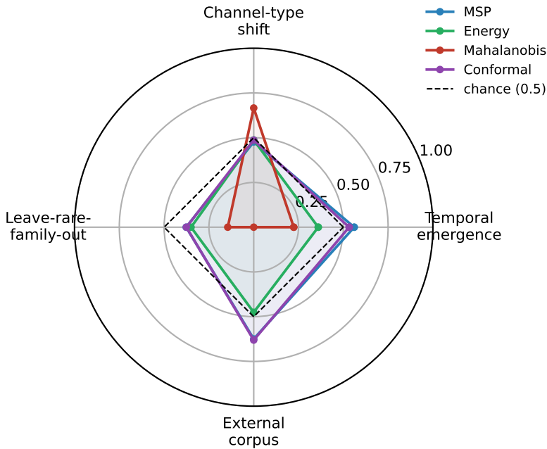
OOD detection AUROC by method and setup (Section 7)
