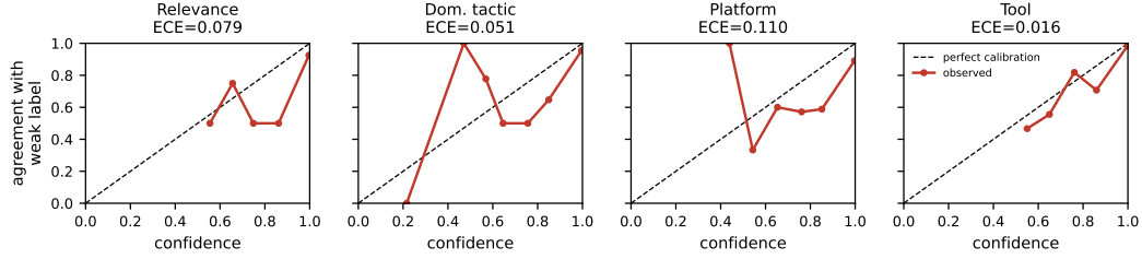
Reliability diagrams against weak labels (Section 5)
