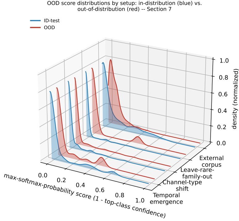
Figure 6: ID-test vs. OOD max-softmax-probability score density per setup, as a 3D ridgeline (kernel density estimate, not binned histograms). Overlap between the blue and red curves is the direct visual counterpart of near-chance AUROC.
